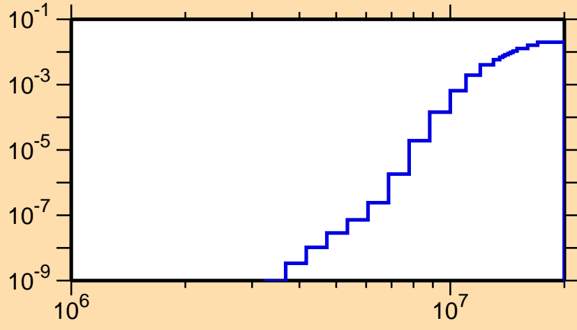
\sigma vs. E for ^{150}\text{Ho}(n,d)
