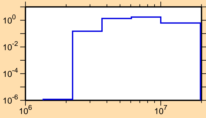
\sigma vs. E for ^{151}\text{Ho}(n,n\text{cont.})
