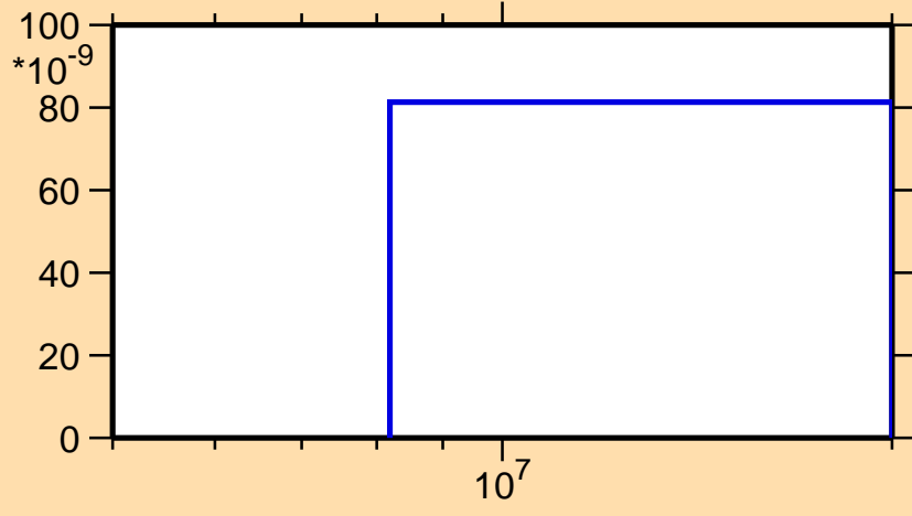
\sigma vs. E for ^{151}\text{Ho}(n,\text{pd})
