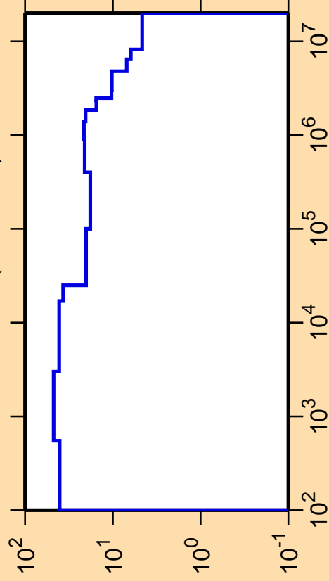
\Delta\sigma/\sigma vs. E for ^{151}\text{Ho}(n,\text{nonel.})
