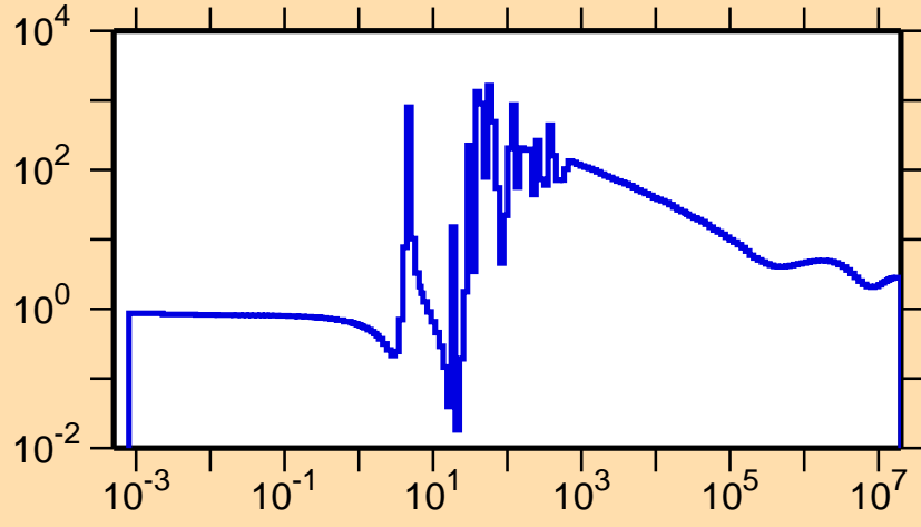
\sigma vs. E for ^{151}\text{Ho}(n,\text{el.})
