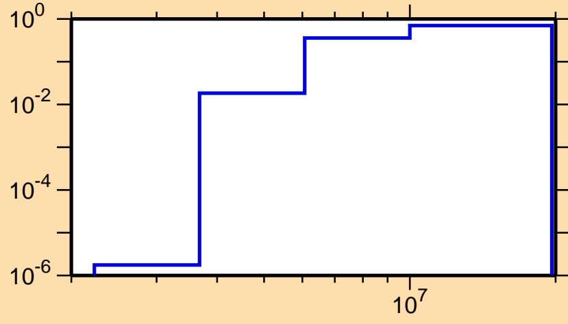
\sigma vs. E for ^{151}\text{Ho}(n,np)
