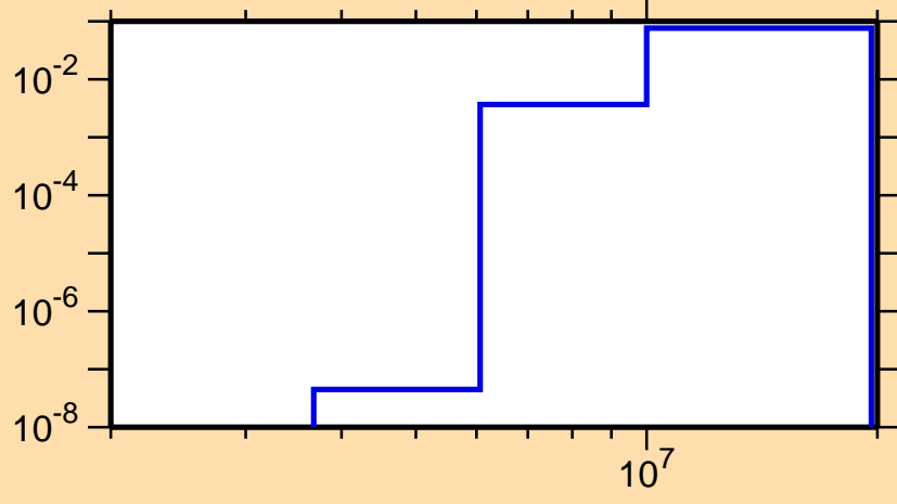
\sigma vs. E for ^{151}\text{Ho}(\text{mt } 45)
