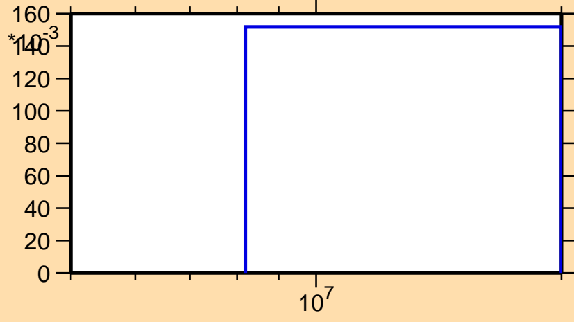
\sigma vs. E for ^{151}\text{Ho}(n,2n\alpha)
