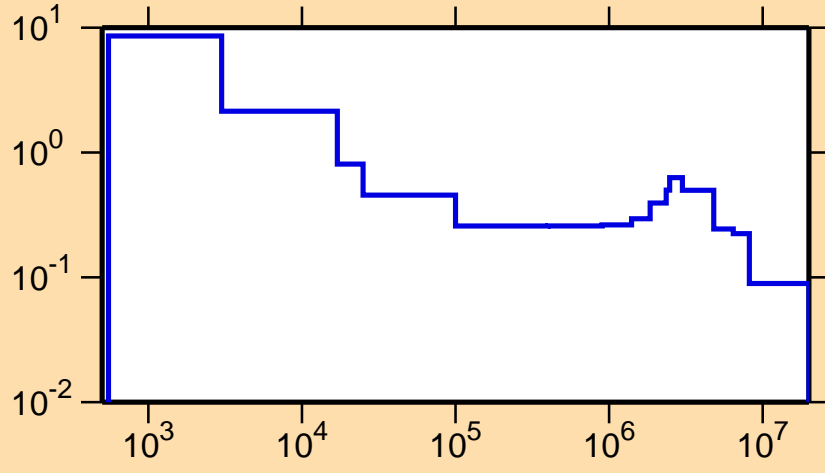
\sigma vs. E for ^{151}\text{Ho}(n,p)
