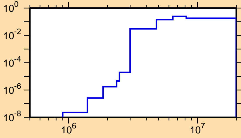
\sigma vs. E for ^{151}\text{Ho}(n,n\alpha)
