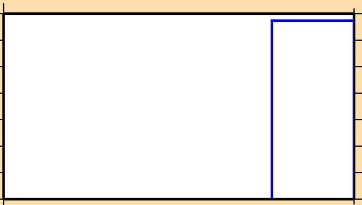
\sigma vs. E for ^{152}\text{Ho}(n,3n)
