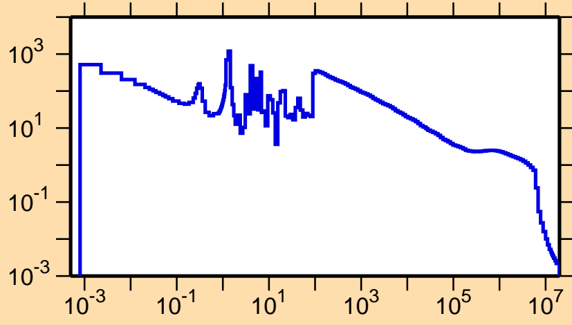
\sigma vs. E for ^{152}\text{Ho}(n,\gamma)
