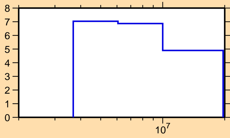
\Delta\sigma/\sigma vs. E for ^{152}\text{Ho}(n,\text{nonel.})
