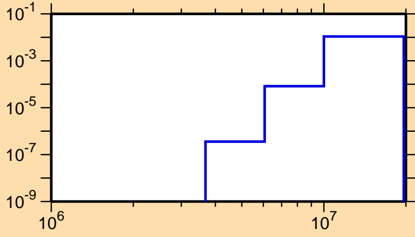
\sigma vs. E for ^{152}\text{Ho}(n,d)
