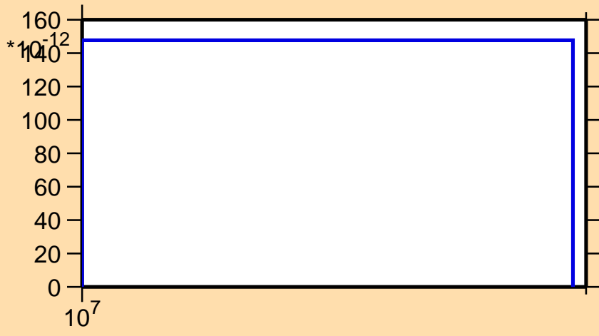
\sigma vs. E for ^{152}\text{Ho} (mt 34)
