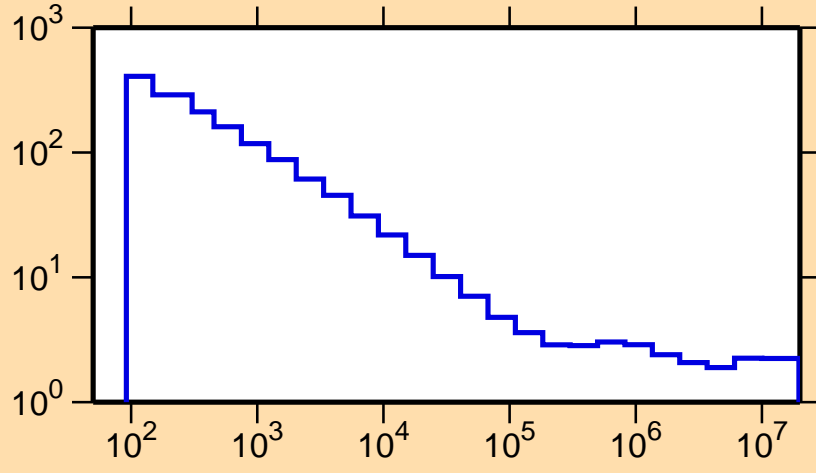
\sigma vs. E for ^{152}\text{Ho}(n,\text{nonel.})
