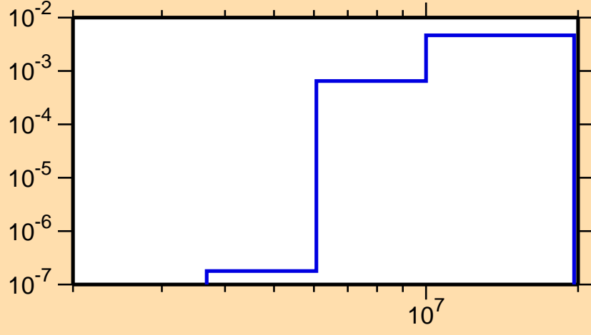
\sigma vs. E for ^{152}\text{Ho}(\text{mt } 45)
