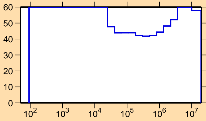
\Delta\sigma/\sigma vs. E for ^{152}\text{Ho}(n,p)
