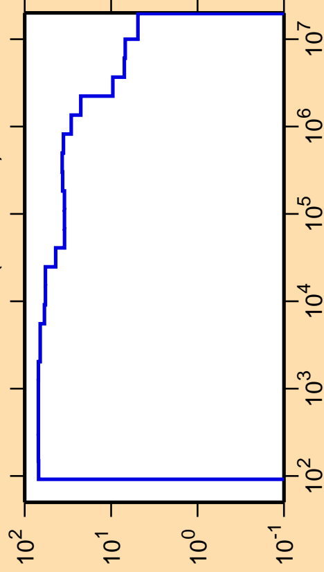
\Delta\sigma/\sigma vs. E for ^{152}\text{Ho}(n,\text{nonel.})
