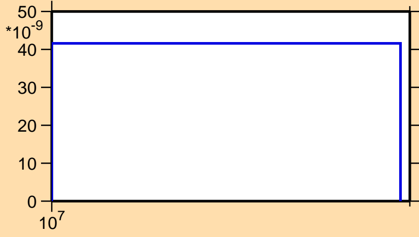
\sigma vs. E for ^{152}\text{Ho}(n,3n\alpha)
