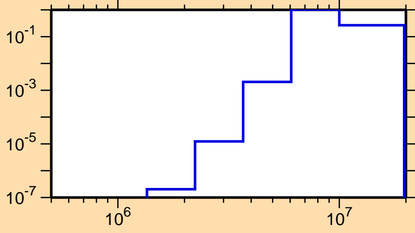
\sigma vs. E for ^{152}\text{Ho}(n,n\alpha)
