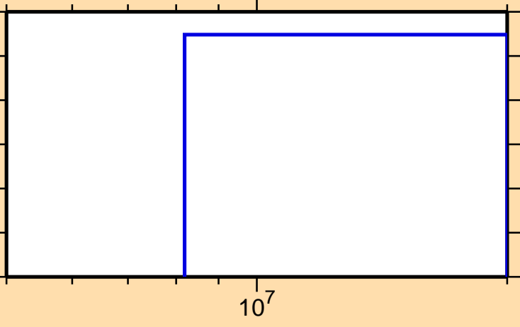
\sigma vs. E for ^{152}\text{Ho}(n,\text{nd})
