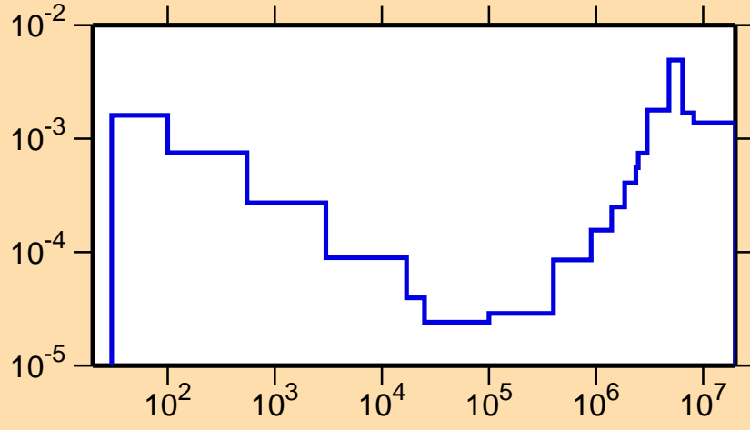
\sigma vs. E for ^{152}\text{Ho}(n,p\alpha)
