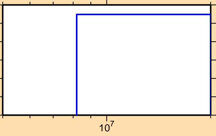
\sigma vs. E for ^{152}\text{Ho}(n,3n)
