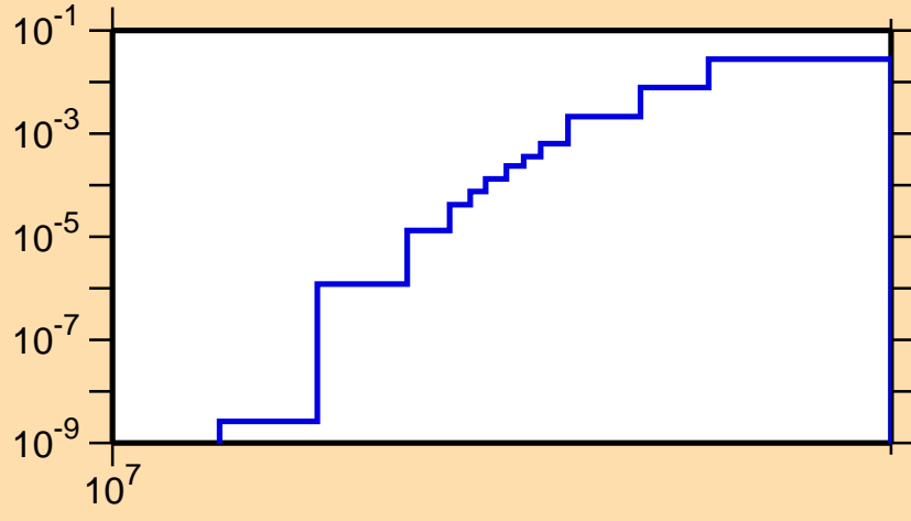
\sigma vs. E for ^{152}\text{Ho}(n,2np)
