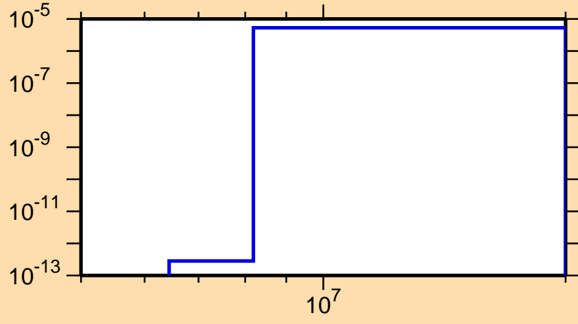
\sigma vs. E for ^{152}\text{Ho}(n,\text{He3})
