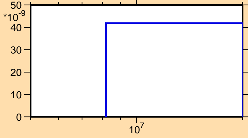
\sigma vs. E for ^{152}\text{Ho}(n,3n\alpha)
