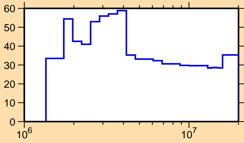
\Delta\sigma/\sigma vs. E for ^{153}\text{Ho}(n,n\text{cont.})
