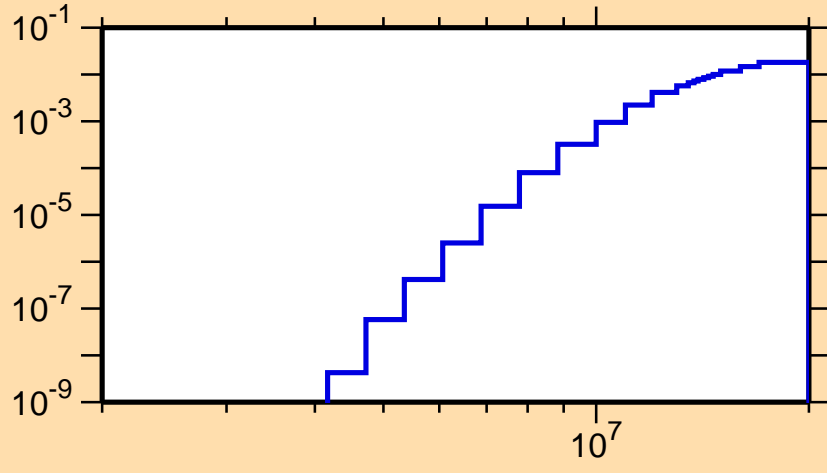
\sigma vs. E for ^{153}\text{Ho}(n,d)
