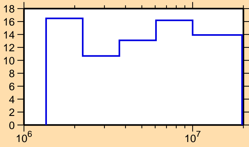
\Delta\sigma/\sigma vs. E for ^{153}\text{Ho}(n,n\text{onel.})
