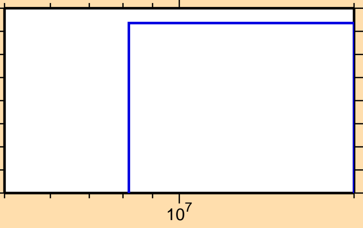
\sigma vs. E for ^{153}\text{Ho}(n,2np)
