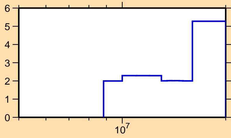
\Delta\sigma/\sigma vs. E for ^{153}\text{Ho}(n,\text{tot.})
