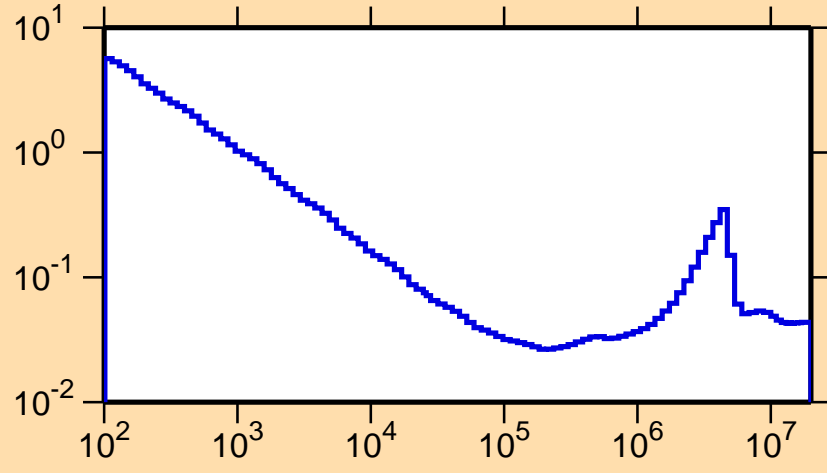
\sigma vs. E for ^{153}\text{Ho}(n,p)
