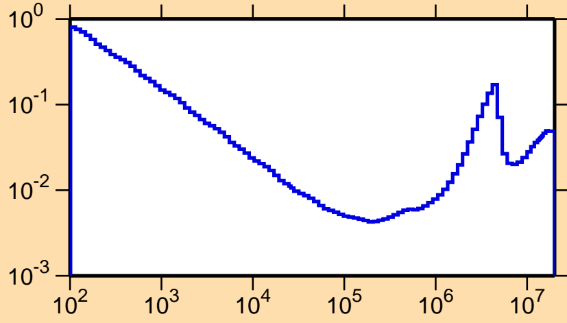
\sigma vs. E for ^{153}\text{Ho}(n,\alpha)
