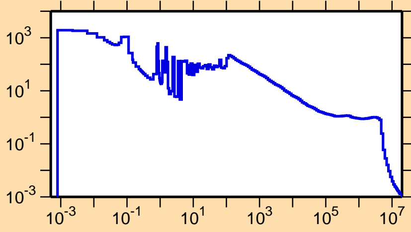
\sigma vs. E for ^{153}\text{Ho}(n,\gamma)
