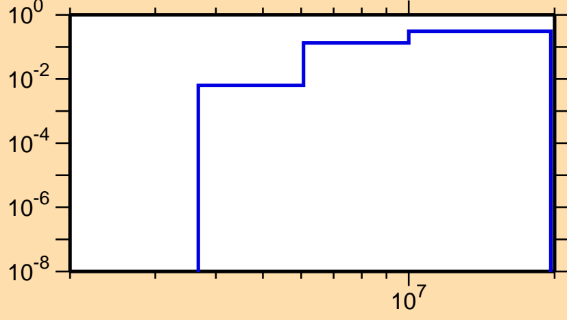
\sigma vs. E for ^{153}\text{Ho}(n,np)
