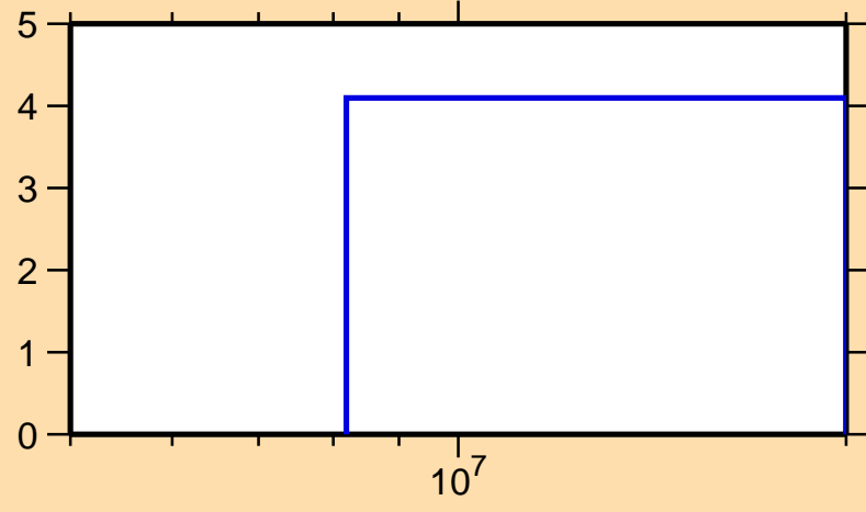
\Delta\sigma/\sigma vs. E for ^{153}\text{Ho}(n,\text{el.})
