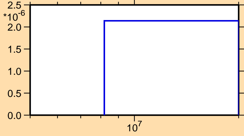
\sigma vs. E for ^{153}\text{Ho}(n,\text{nd})
