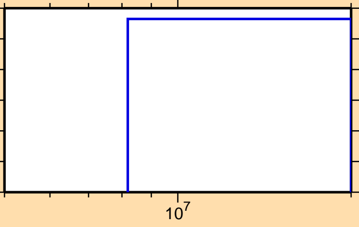
\sigma vs. E for ^{153}\text{Ho}(n,nt)
