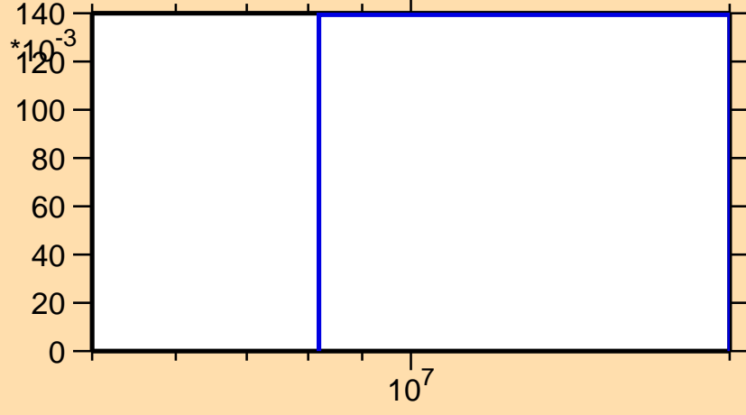
\sigma vs. E for ^{153}\text{Ho}(n,2n\alpha)
