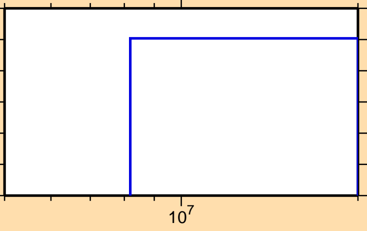
\sigma vs. E for ^{153}\text{Ho}(n,3n)
