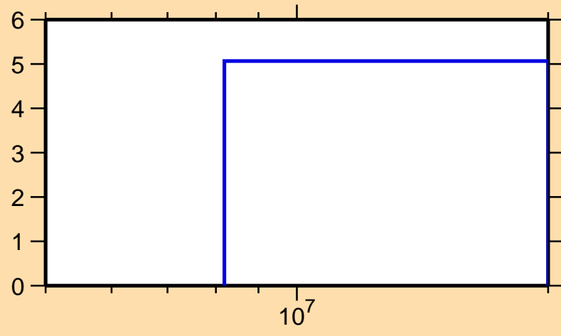
\Delta\sigma/\sigma vs. E for ^{153}\text{Ho}(n,\text{nonel.})
