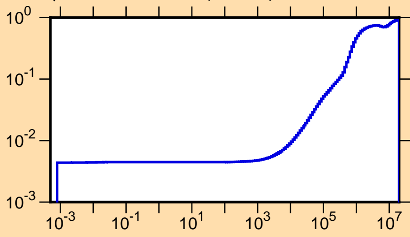
\mu vs. E for ^{154}\text{Ho}(\text{mt251})
