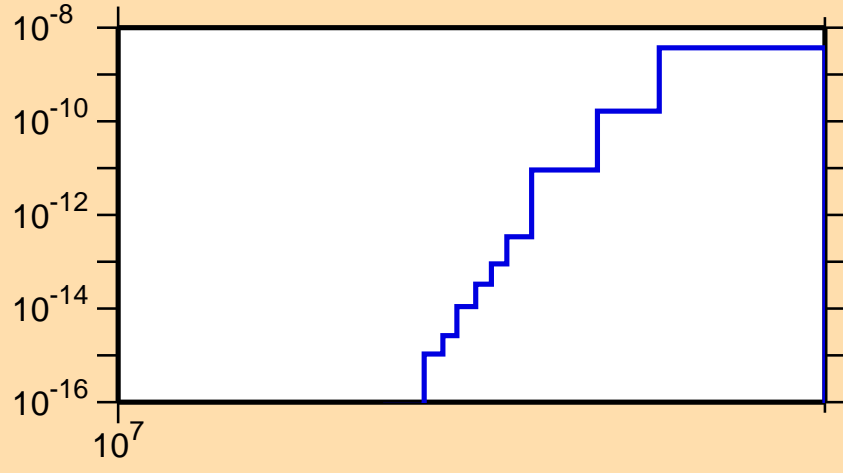
\sigma vs. E for ^{154}\text{Ho}(n,\text{pt})
