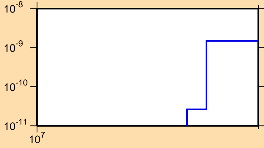
\sigma vs. E for ^{154}\text{Ho} (mt 34)
