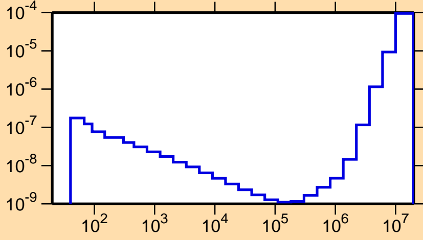
\sigma vs. E for ^{154}\text{Ho}(n,p\alpha)
