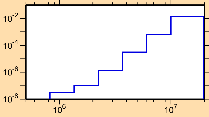
\sigma vs. E for ^{154}\text{Ho}(n,n\alpha)
