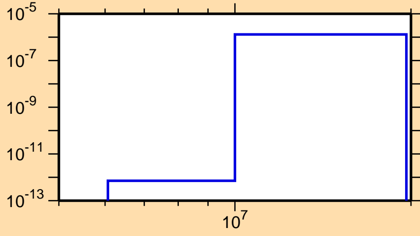
\sigma vs. E for ^{154}\text{Ho}(n,\text{He3})
