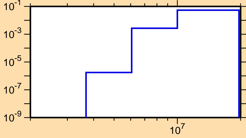
\sigma vs. E for ^{154}\text{Ho}(n,np)
