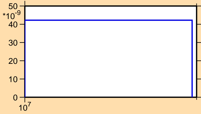
\sigma vs. E for ^{154}\text{Ho}(n,nt)
