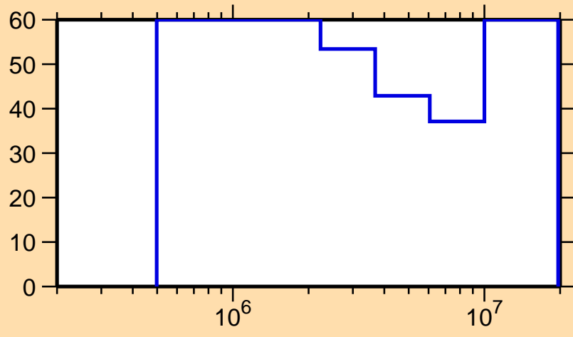
\Delta\sigma/\sigma vs. E for ^{154}\text{Ho}(n,n\text{cont.})
