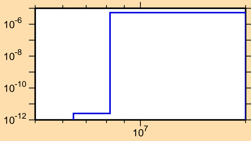
\sigma vs. E for ^{154}\text{Ho} (mt 45)
