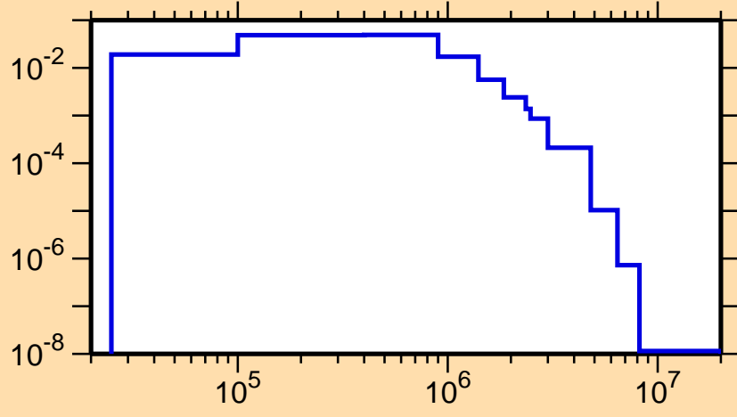
\sigma vs. E for ^{154}\text{Ho}(n,n_1)
