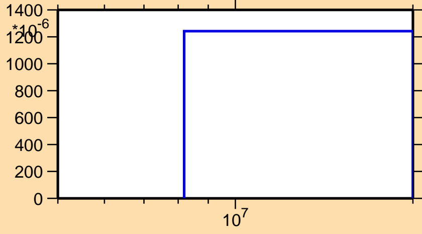
\sigma vs. E for ^{154}\text{Ho}(n,2np)
