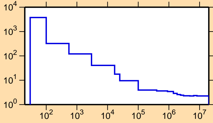
\sigma vs. E for ^{154}\text{Ho}(n,\text{nonel.})
