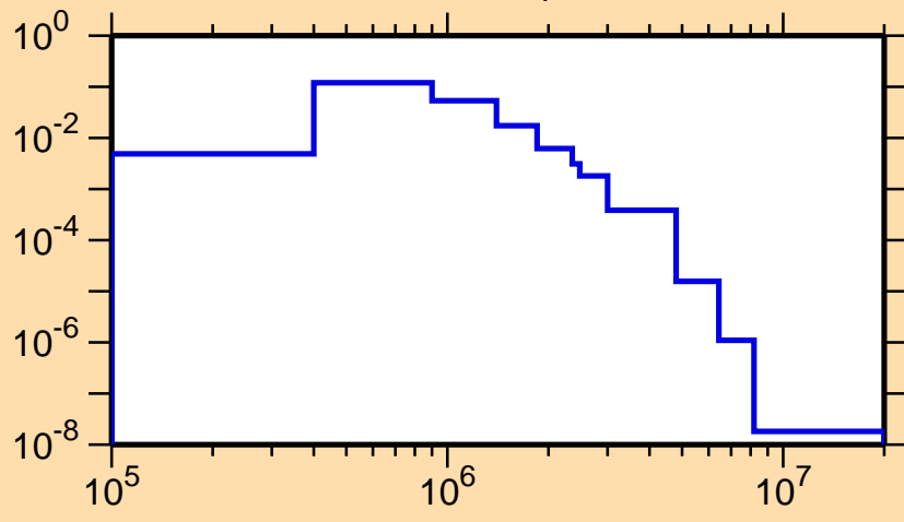
\sigma vs. E for ^{154}\text{Ho}(n,n_4)
