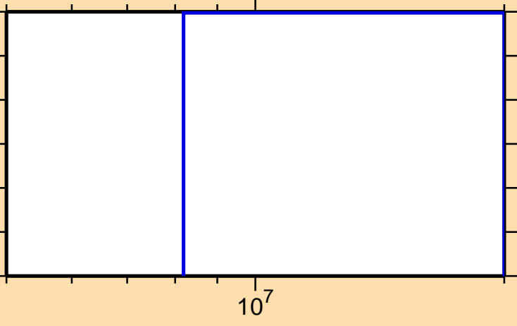
\sigma vs. E for ^{154}\text{Ho}(n,3n)
