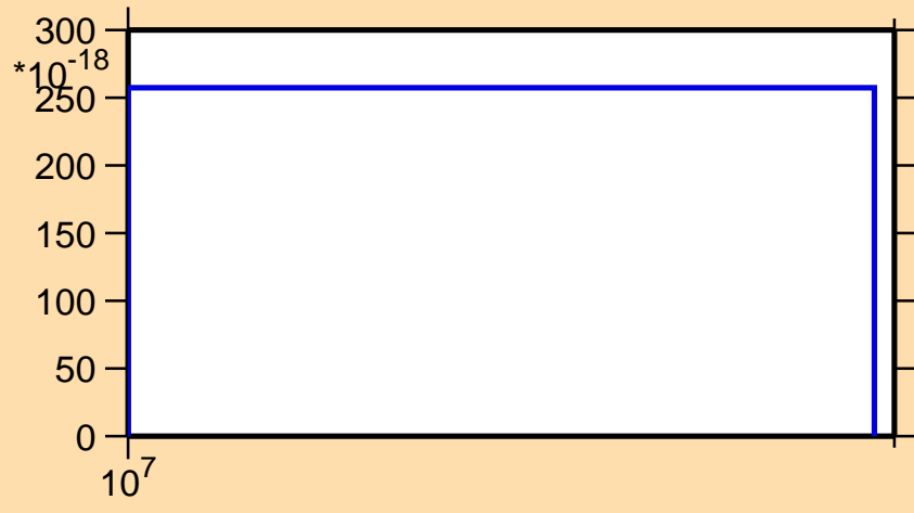
\sigma vs. E for ^{154}\text{Ho} (mt 11)
