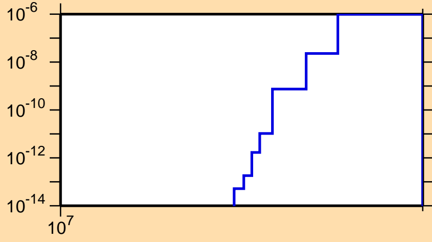
\sigma vs. E for ^{155}\text{Ho}(n,nt)
