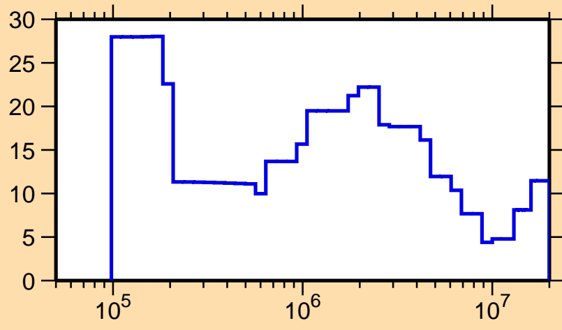
\Delta\sigma/\sigma vs. E for ^{155}\text{Ho}(n,\text{tot.})
