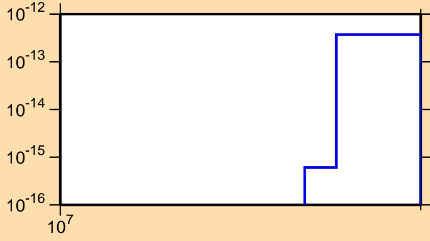
\sigma vs. E for ^{155}\text{Ho}(n,\text{pt})
