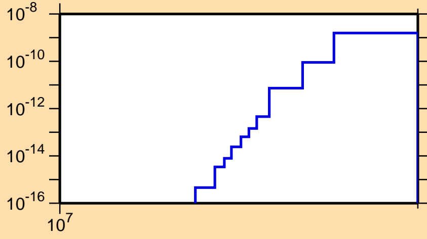
\sigma vs. E for ^{155}\text{Ho}(n,\text{pd})
