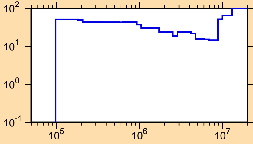
\Delta\sigma/\sigma vs. E for ^{155}\text{Ho}(n,\text{inel.})
