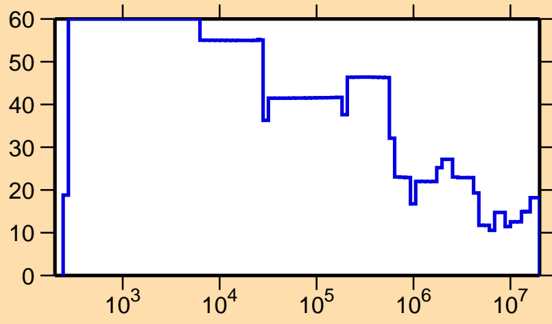
\Delta\sigma/\sigma vs. E for ^{155}\text{Ho}(n,\text{el.})
