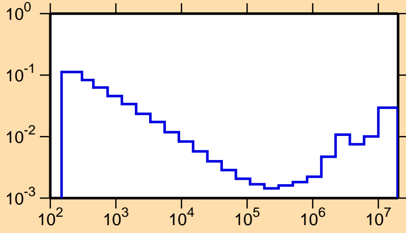
\sigma vs. E for ^{155}\text{Ho}(n,p)
