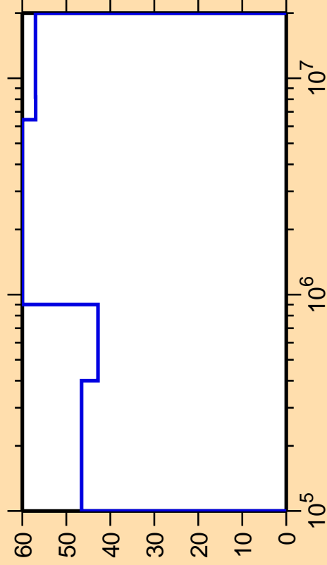
\Delta\sigma/\sigma vs. E for ^{155}\text{Ho}(n,n_1)
