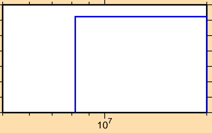
\sigma vs. E for ^{155}\text{Ho}(\text{mt117})
