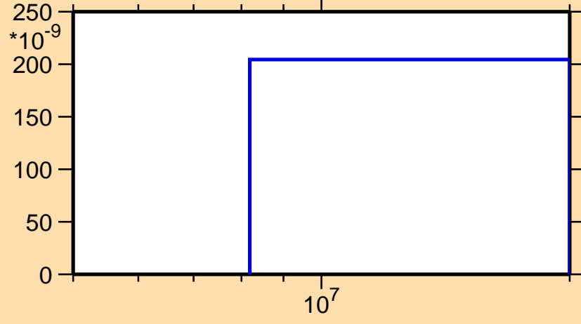
\sigma vs. E for ^{155}\text{Ho} (mt 45)
