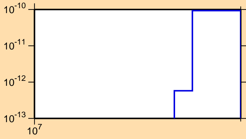
\sigma vs. E for ^{156}\text{Ho} (mt 34)
