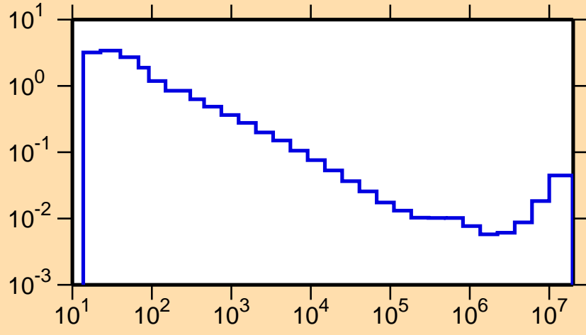
\sigma vs. E for ^{156}\text{Ho}(n,p)
