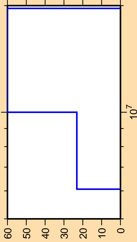
\Delta\sigma/\sigma vs. E for ^{156}\text{Ho}(n,2n\alpha)
