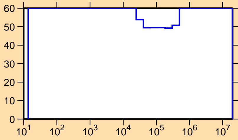
\Delta\sigma/\sigma vs. E for ^{156}\text{Ho}(n,\gamma)
