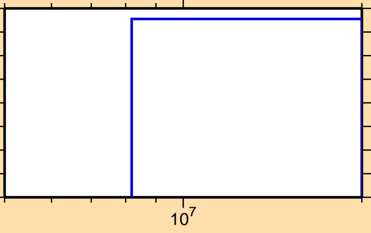
\sigma vs. E for ^{156}\text{Ho}(n,2n\alpha)
