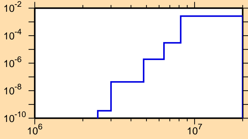
\sigma vs. E for ^{156}\text{Ho}(n,n\alpha)
