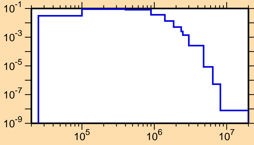
\sigma vs. E for ^{156}\text{Ho}(n,n_3)
