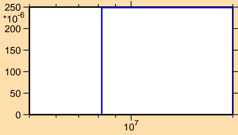
\sigma vs. E for ^{156}\text{Ho}(n,2n\alpha)
