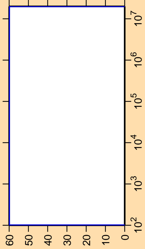
\Delta\sigma/\sigma vs. E for ^{156}\text{Ho}(n,\alpha)
