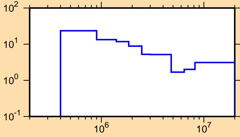
\Delta\sigma/\sigma vs. E for ^{156}\text{Ho}(n,n\text{onel.})
