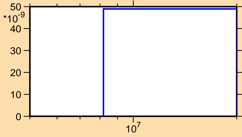
\sigma vs. E for ^{156}\text{Ho} (mt 45)
