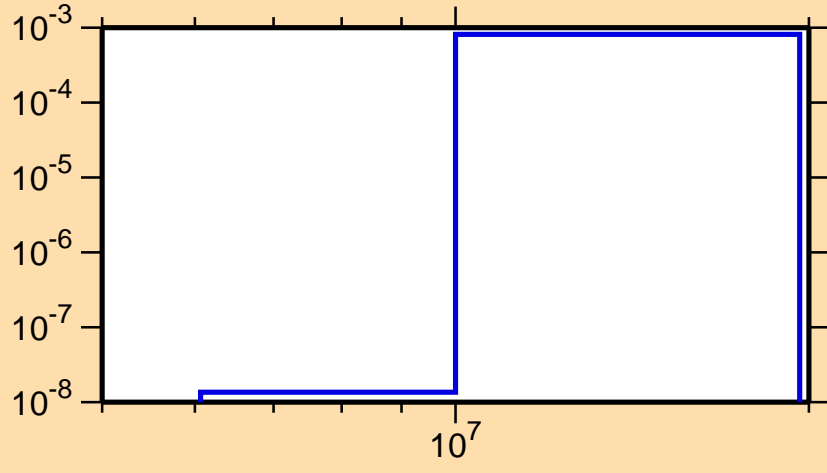
\sigma vs. E for ^{156}\text{Ho}(n,t)
