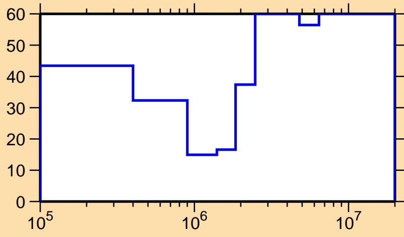
\Delta\sigma/\sigma vs. E for ^{156}\text{Ho}(n,n_1)
