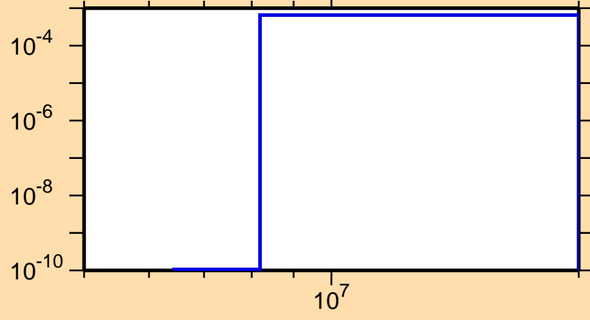
\sigma vs. E for ^{156}\text{Ho}(n,t)
