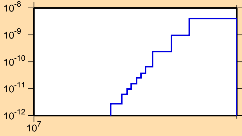
\sigma vs. E for ^{157}\text{Ho}(\text{mt117})
