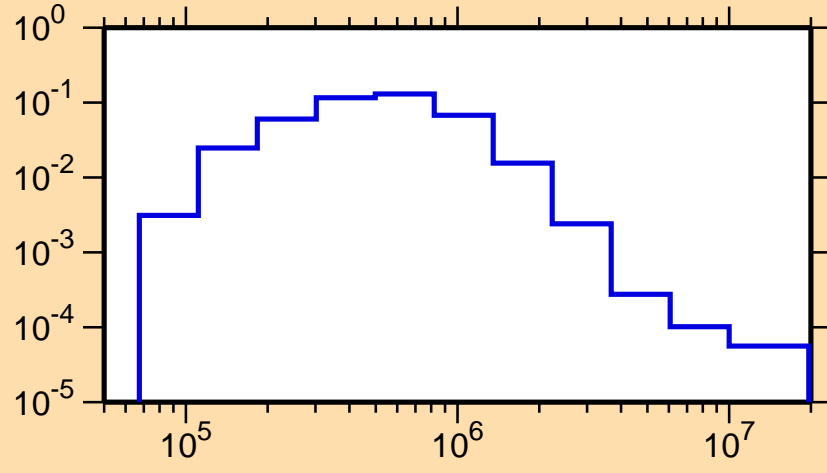
\sigma vs. E for ^{157}\text{Ho}(n,n_4)
