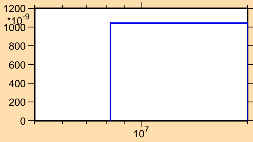
\sigma vs. E for ^{157}\text{Ho}(n,2np)
