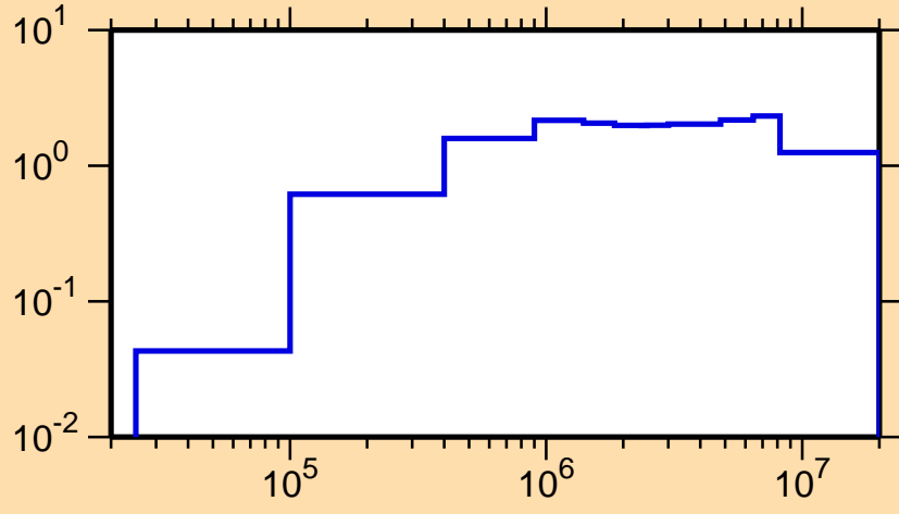
\sigma vs. E for ^{157}\text{Ho}(n,\text{inel.})
