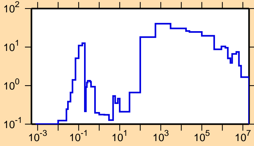
\Delta\sigma/\sigma vs. E for ^{157}\text{Ho}(n,\text{tot.})
