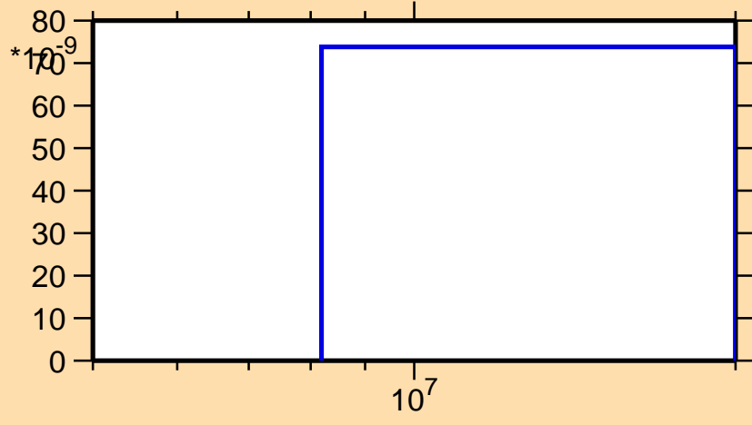
\sigma vs. E for ^{157}\text{Ho}(n,\text{nd})
