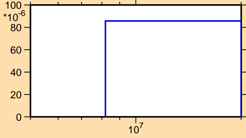
\sigma vs. E for ^{157}\text{Ho}(n,t)
