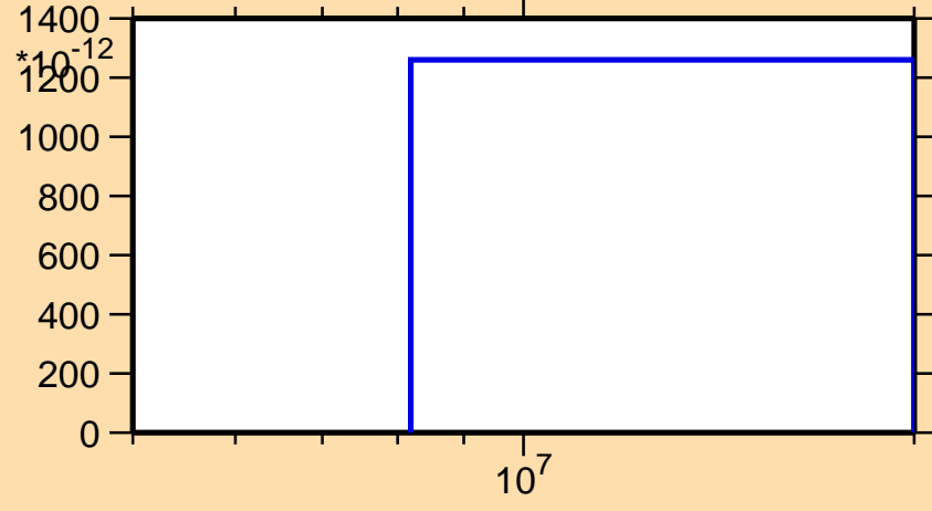
\sigma vs. E for ^{157}\text{Ho} (mt 45)
