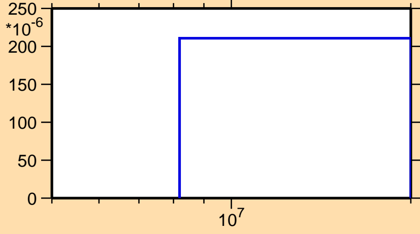
\sigma vs. E for ^{157}\text{Ho}(n,3n)
