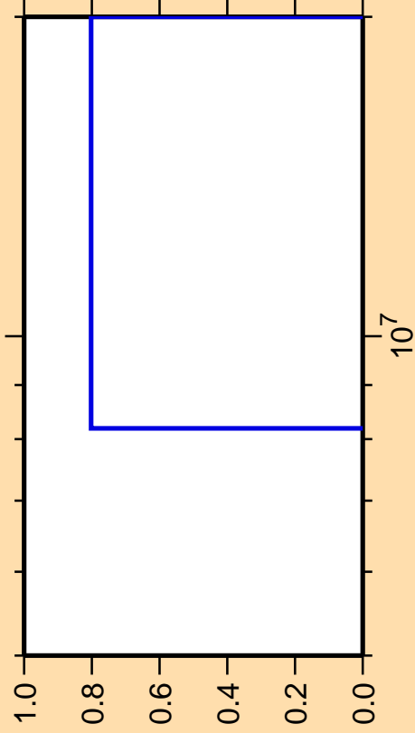
\Delta\sigma/\sigma vs. E for ^{157}\text{Ho}(n,3n\alpha)
