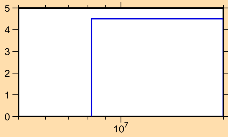
\Delta\sigma/\sigma vs. E for ^{157}\text{Ho}(n,\text{nonel.})
