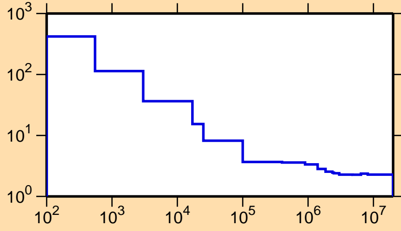
\sigma vs. E for ^{157}\text{Ho}(n,\text{nonel.})
