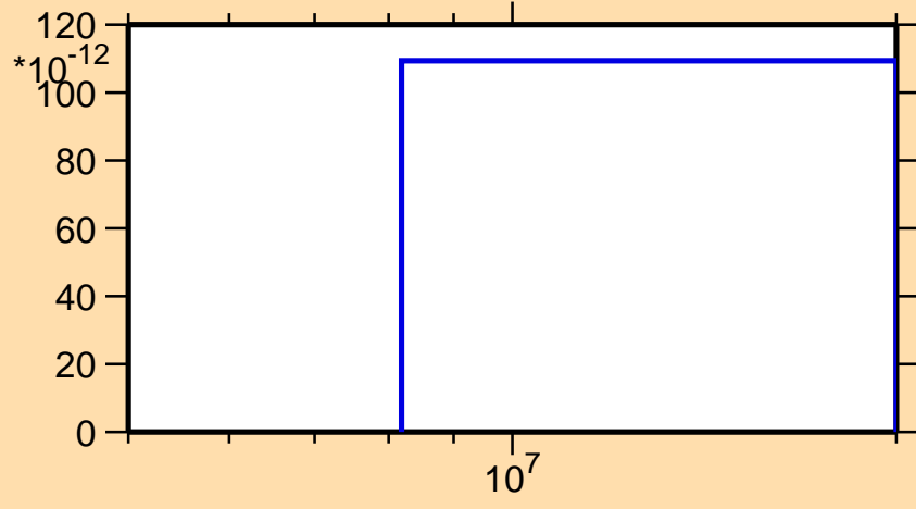
\sigma vs. E for ^{157}\text{Ho}(\text{mt117})
