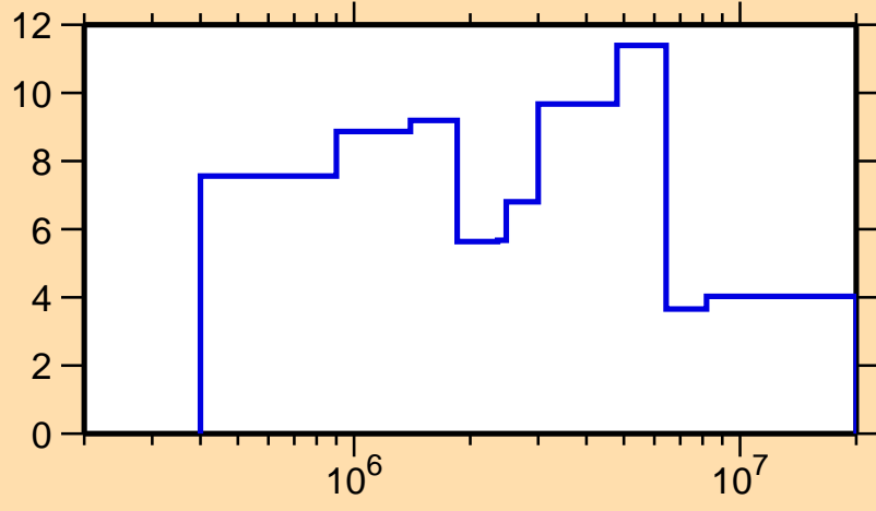
\Delta\sigma/\sigma vs. E for ^{157}\text{Ho}(n,\text{el.})
