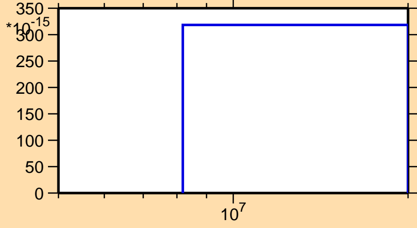
\sigma vs. E for ^{157}\text{Ho}(n,pd)
