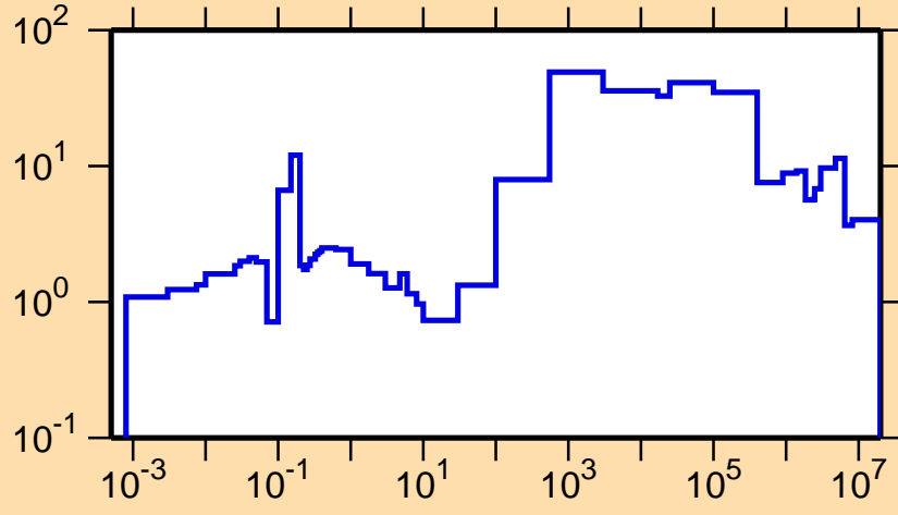
\Delta\sigma/\sigma vs. E for ^{157}\text{Ho}(n,\text{el.})
