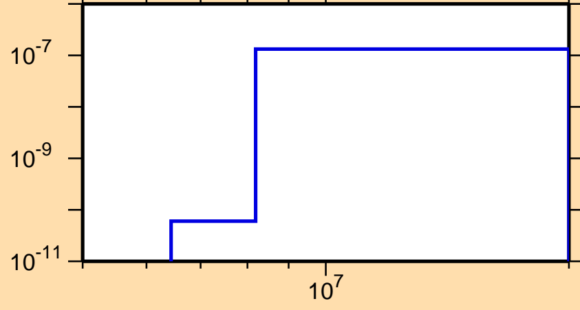
\sigma vs. E for ^{157}\text{Ho}(n,p\alpha)
