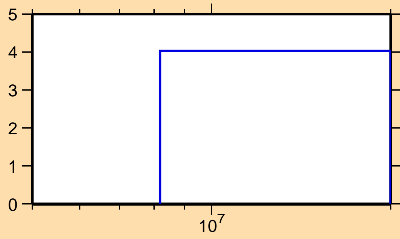
\Delta\sigma/\sigma vs. E for ^{157}\text{Ho}(n,\text{el.})
