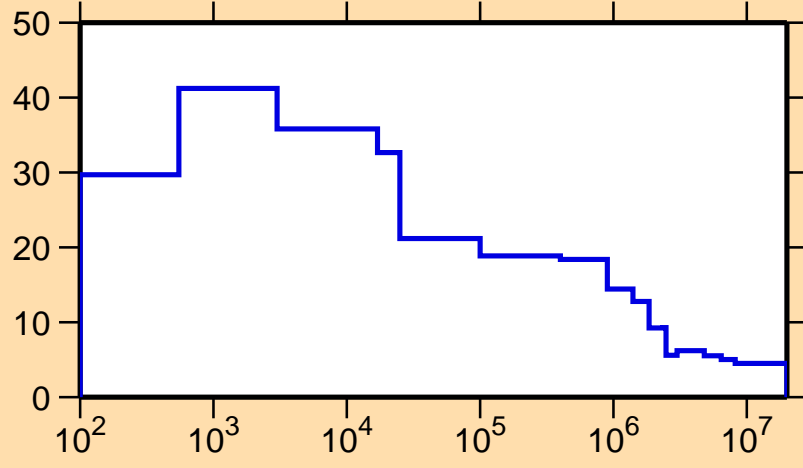
\Delta\sigma/\sigma vs. E for ^{157}\text{Ho}(n,\text{nonel.})
