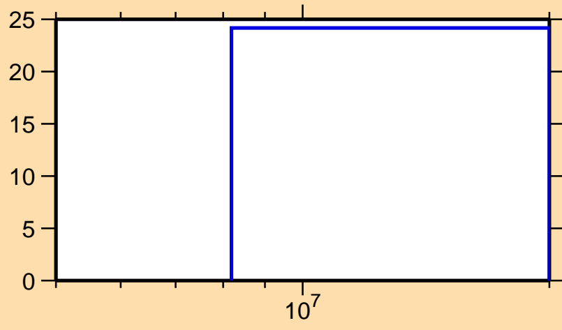
\Delta\sigma/\sigma vs. E for ^{157}\text{Ho}(n,\text{inel.})
