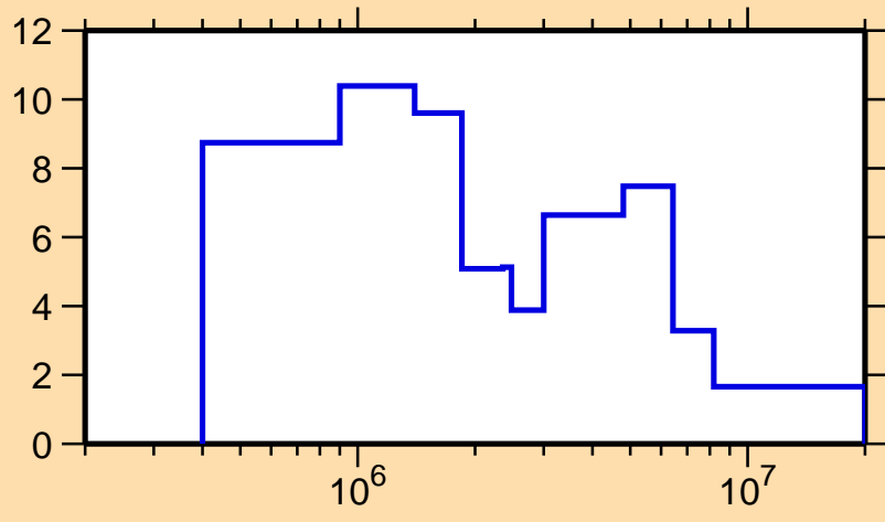
\Delta\sigma/\sigma vs. E for ^{157}\text{Ho}(n,\text{tot.})
