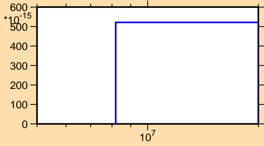
\sigma vs. E for ^{157}\text{Ho}(n,3n\alpha)
