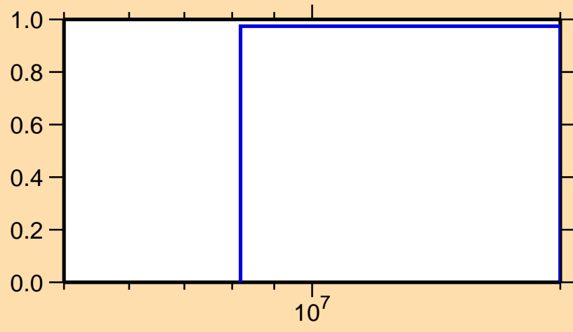
\sigma vs. E for ^{157}\text{Ho}(n,2n)
