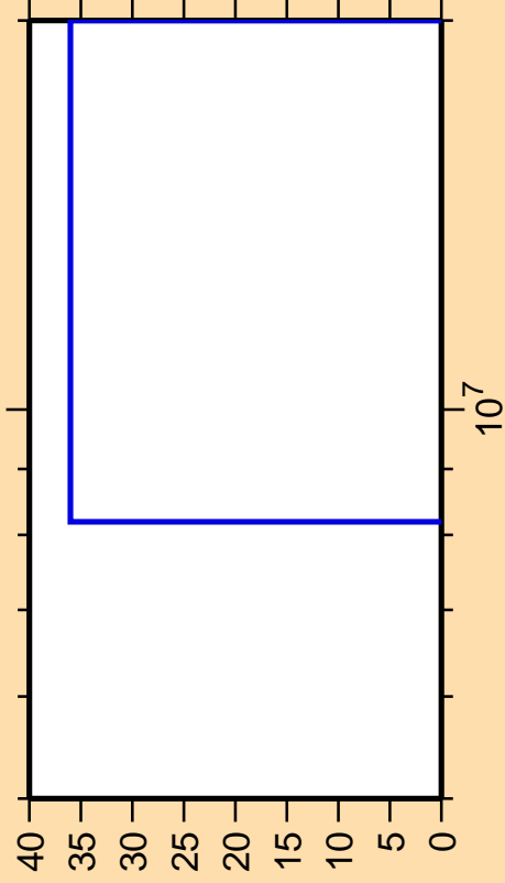
\Delta\sigma/\sigma vs. E for ^{157}\text{Ho}(n,3n)
