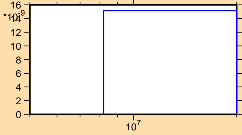
\sigma vs. E for ^{157}\text{Ho}(n,\text{He3})
