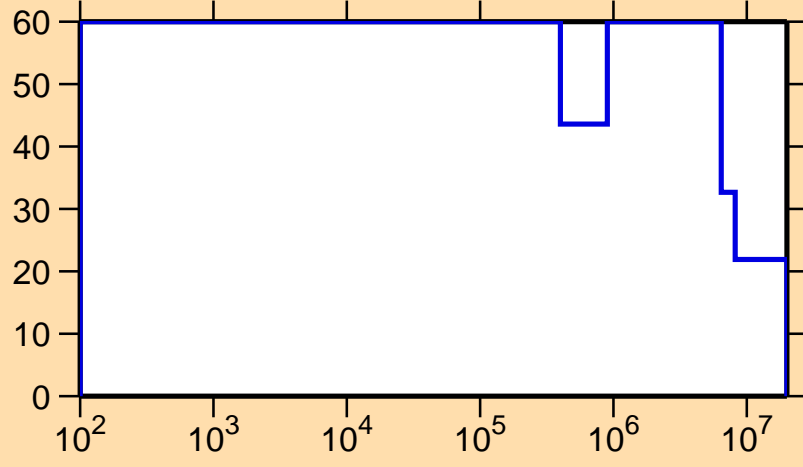
\Delta\sigma/\sigma vs. E for ^{157}\text{Ho}(n,p)
