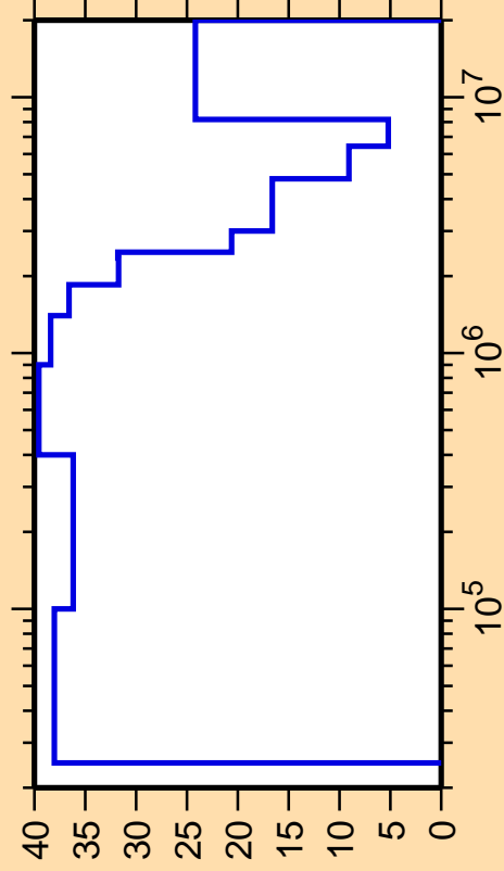
\Delta\sigma/\sigma vs. E for ^{157}\text{Ho}(n,\text{inel.})
