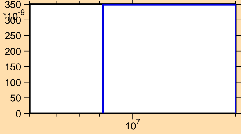
\sigma vs. E for ^{157}\text{Ho}(n,2n\alpha)
