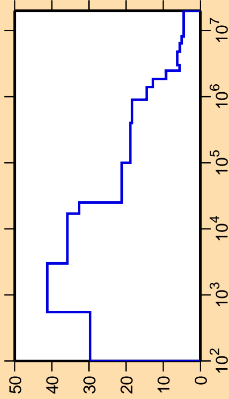
\Delta\sigma/\sigma vs. E for ^{157}\text{Ho}(n,\text{nonel.})
