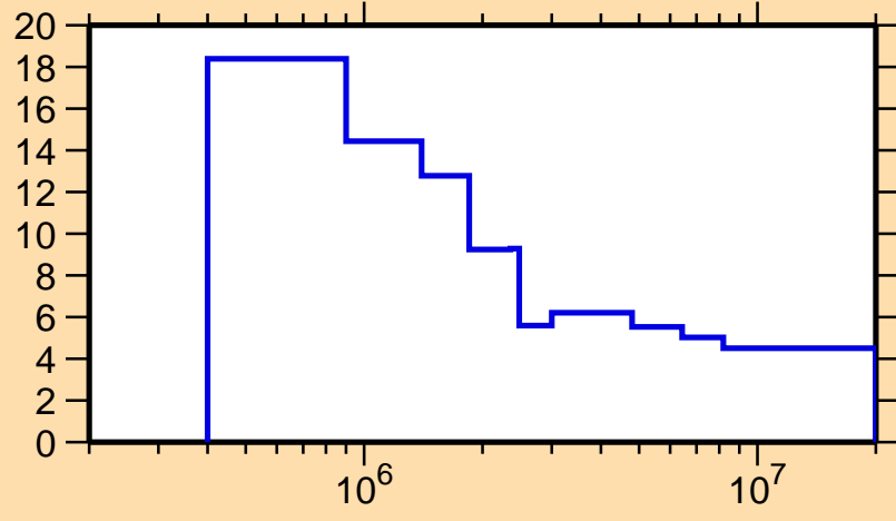
\Delta\sigma/\sigma vs. E for ^{157}\text{Ho}(n,\text{nonel.})
