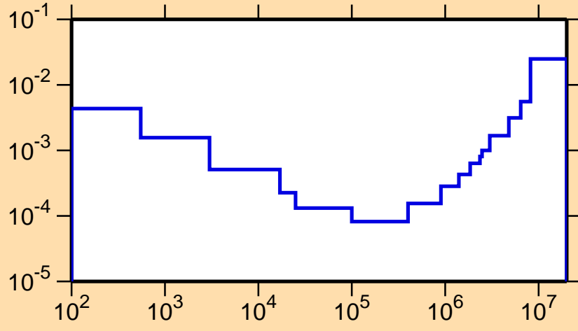
\sigma vs. E for ^{157}\text{Ho}(n,p)
