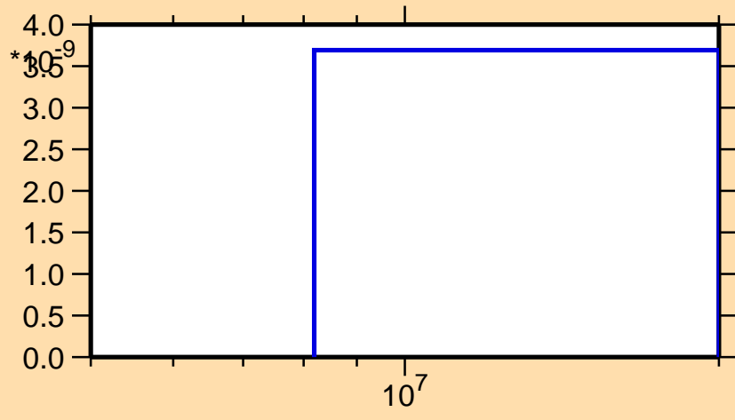
\sigma vs. E for ^{157}\text{Ho}(n,nt)
