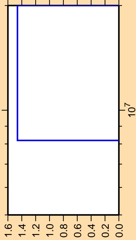
\Delta\sigma/\sigma vs. E for ^{157}\text{Ho}(n,pd)
