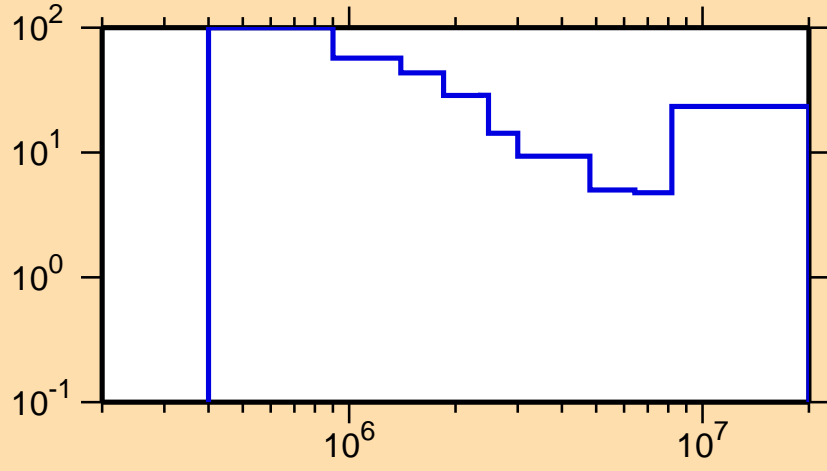
\Delta\sigma/\sigma vs. E for ^{157}\text{Ho}(n,n\text{cont.})
