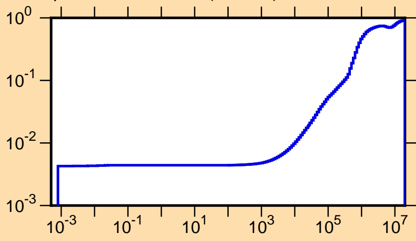
\mu vs. E for ^{158}\text{Ho}(\text{mt251})
