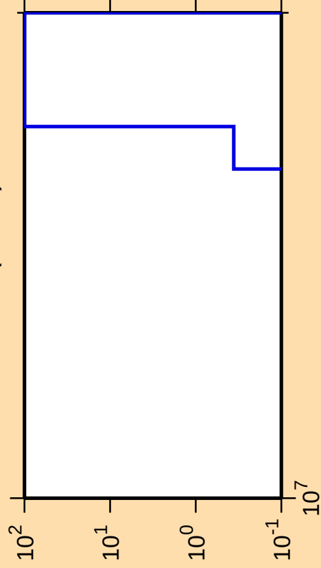
\Delta\sigma/\sigma vs. E for ^{158}\text{Ho}(\text{mt } 34)
