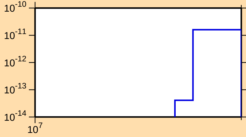
\sigma vs. E for ^{158}\text{Ho}(\text{mt } 34)
