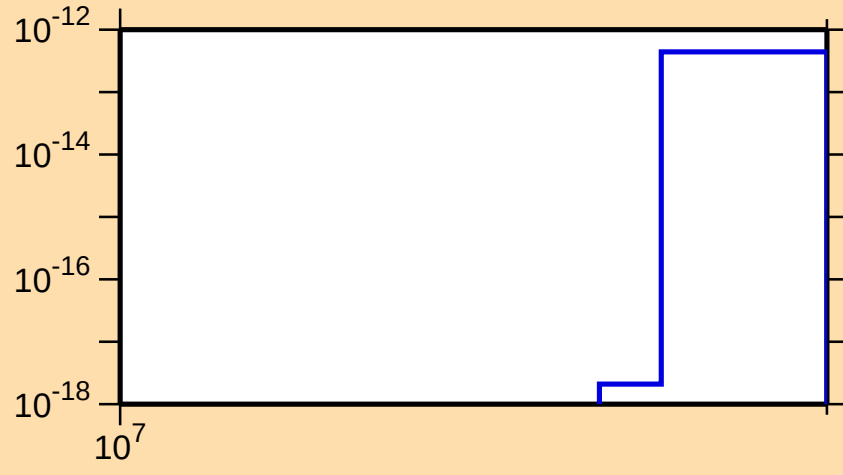
\sigma vs. E for ^{158}\text{Ho}(n,3n\alpha)
