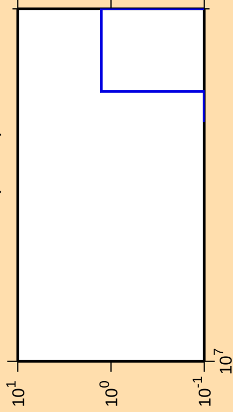
\Delta\sigma/\sigma vs. E for ^{158}\text{Ho}(n,3n\alpha)
