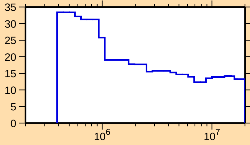
\Delta\sigma/\sigma vs. E for ^{158}\text{Ho}(n,n\text{oncl.})
