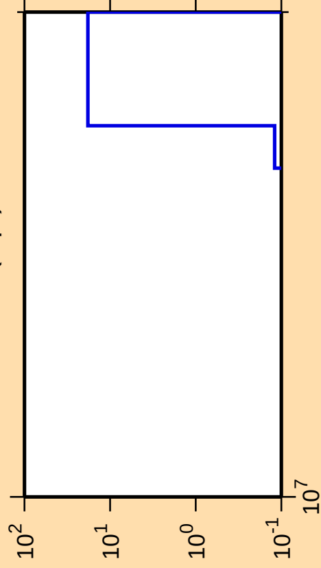
\Delta\sigma/\sigma vs. E for ^{158}\text{Ho}(n,\text{pt})
