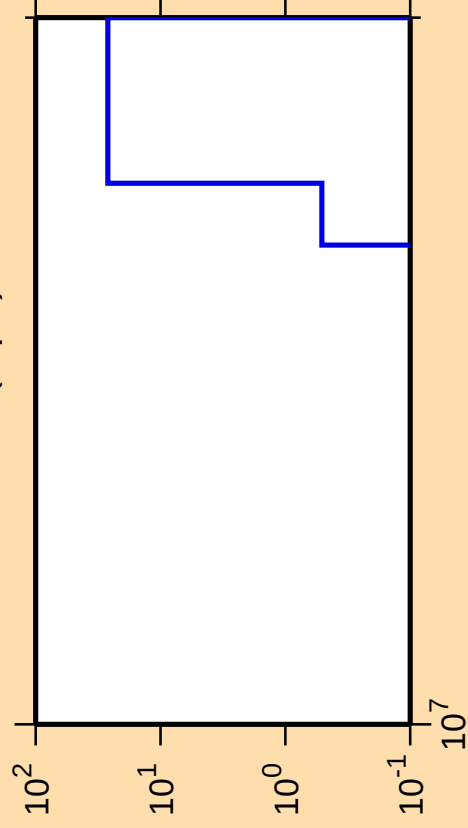
\Delta\sigma/\sigma vs. E for ^{158}\text{Ho}(n,\text{pd})
