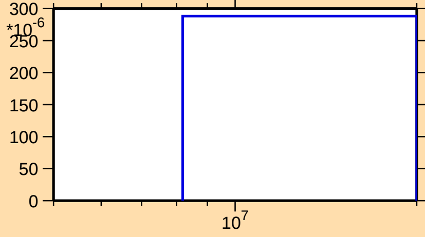
\sigma vs. E for ^{158}\text{Ho}(n,3n)
