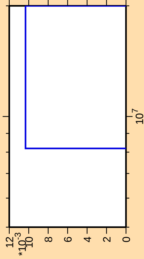
\Delta\sigma/\sigma vs. E for ^{158}\text{Ho}(n,3n\alpha)
