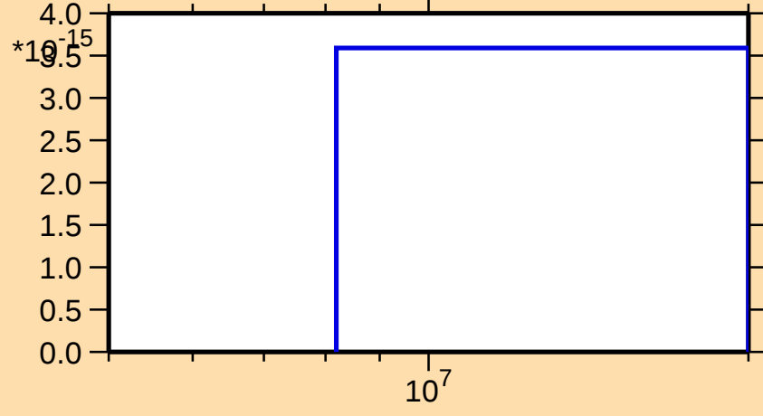
\sigma vs. E for ^{158}\text{Ho}(n,3n\alpha)
