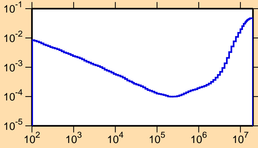
\sigma vs. E for ^{158}\text{Ho}(n,p)
