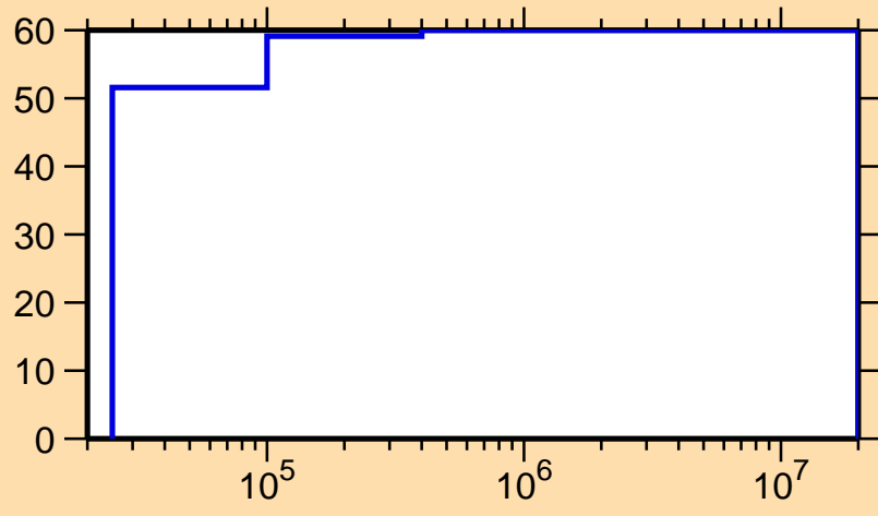
\Delta\sigma/\sigma vs. E for ^{158}\text{Ho}(n,n_1)
