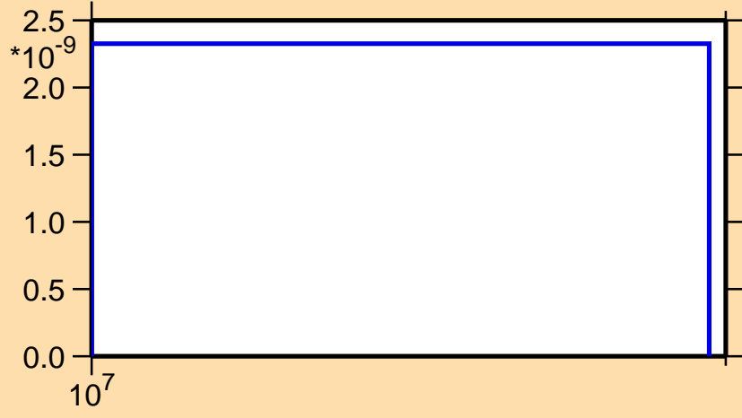
\sigma vs. E for ^{159}\text{Ho}(n,nt)
