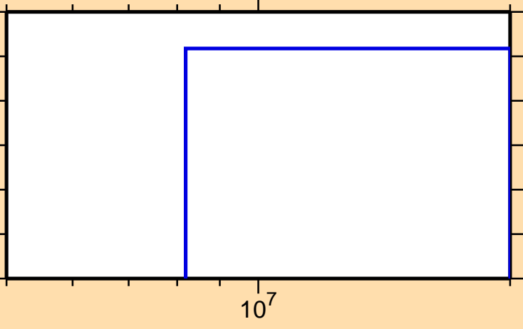
\sigma vs. E for ^{159}\text{Ho}(n,2n\alpha)
