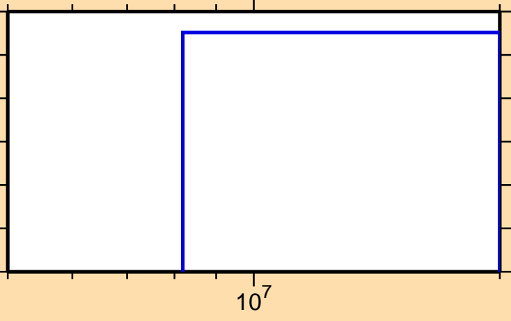
\sigma vs. E for ^{159}\text{Ho} (mt 45)
