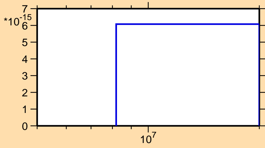
\sigma vs. E for ^{159}\text{Ho}(n,\text{pd})
