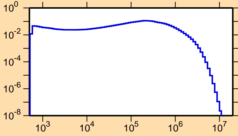
\sigma vs. E for ^{159}\text{Ho}(n,n_1)
