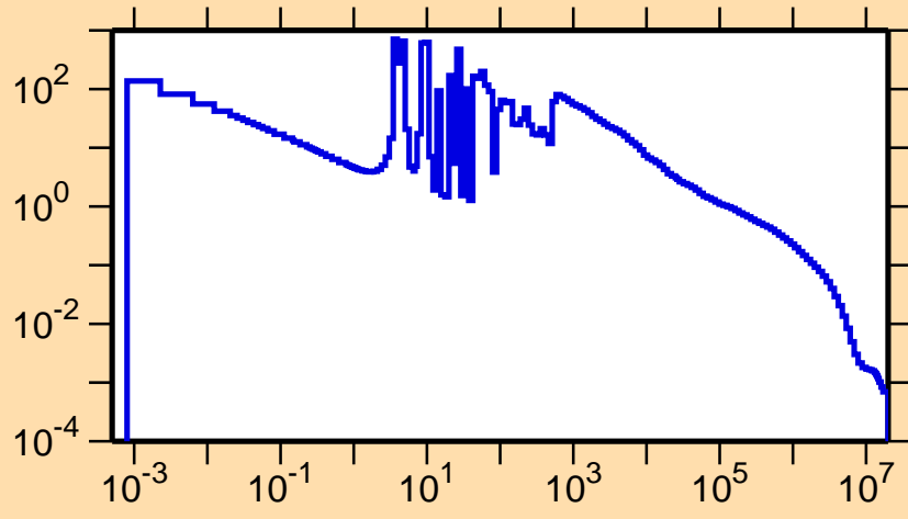
\sigma vs. E for ^{159}\text{Ho}(n,\gamma)
