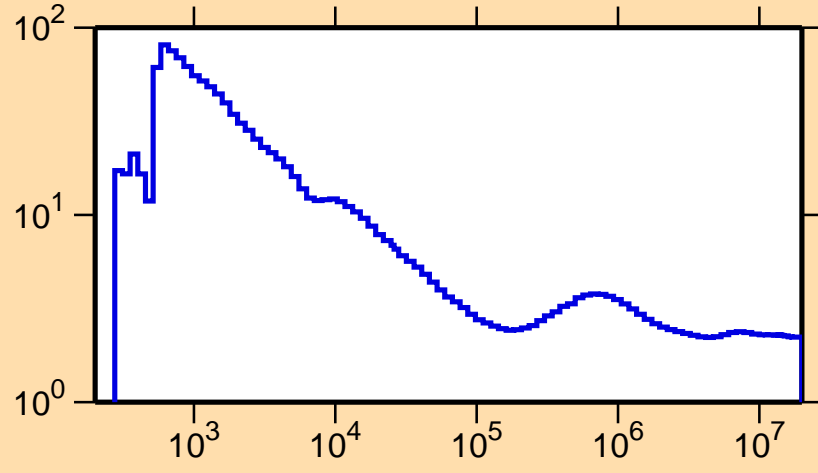
\sigma vs. E for ^{159}\text{Ho}(n,\text{nonel.})
