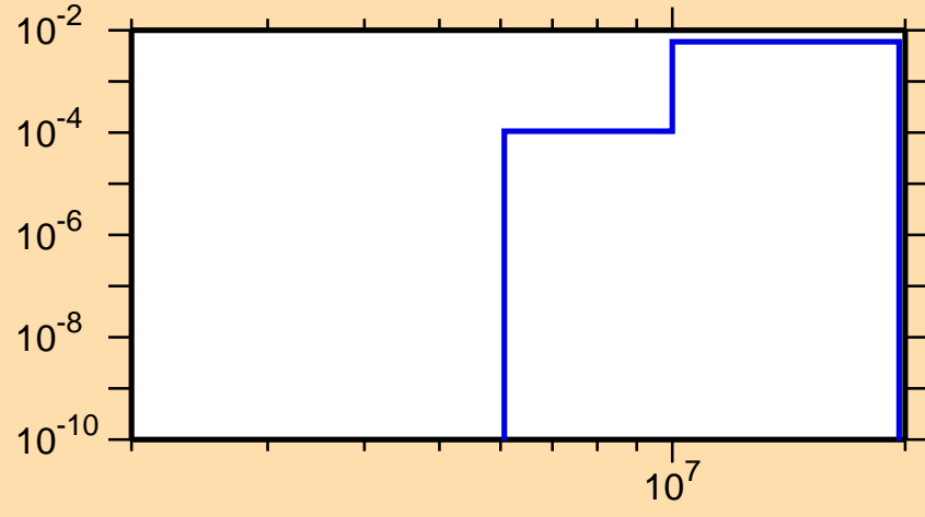
\sigma vs. E for ^{159}\text{Ho}(n,np)
