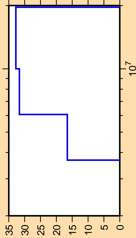
\Delta\sigma/\sigma vs. E for ^{159}\text{Ho}(n,np)
