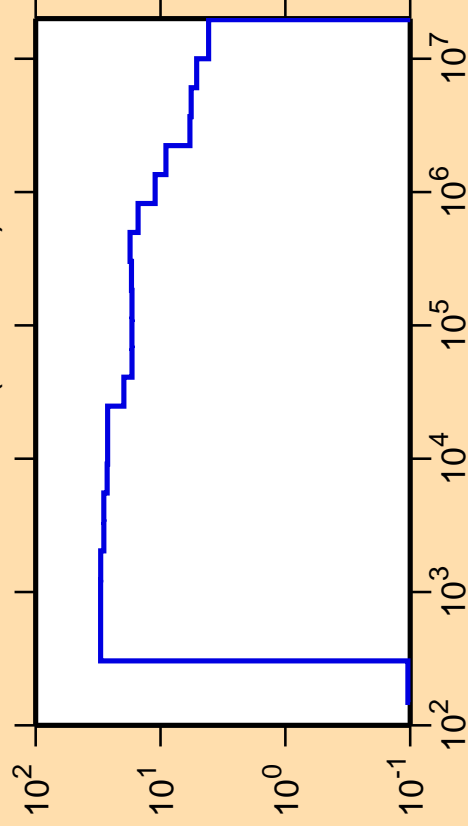
\Delta\sigma/\sigma vs. E for ^{159}\text{Ho}(n,\text{nonel.})
