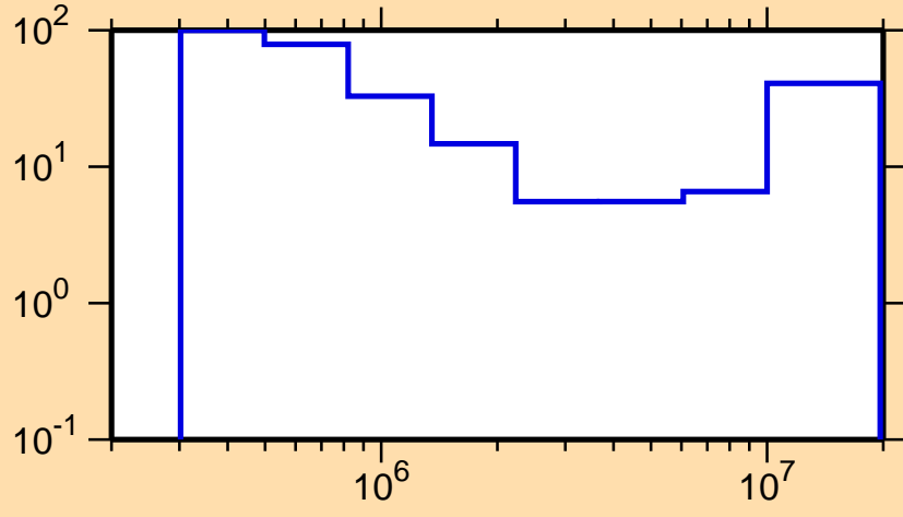
\Delta\sigma/\sigma vs. E for ^{159}\text{Ho}(n,n\text{cont.})
