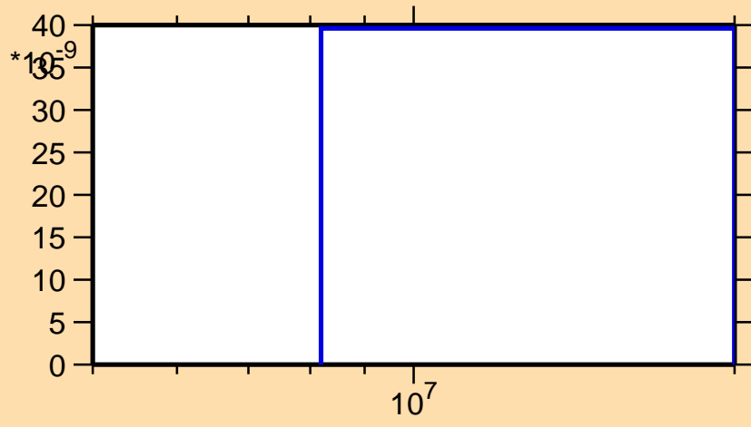
\sigma vs. E for ^{159}\text{Ho}(n,2n\alpha)
