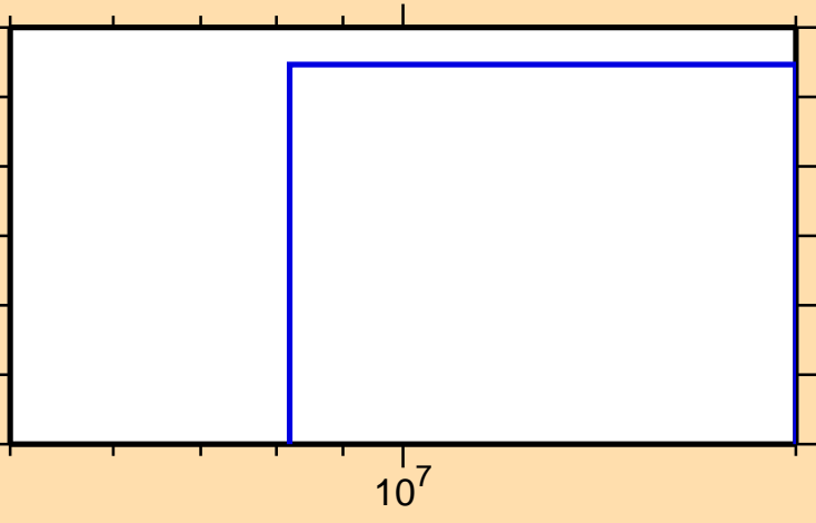
\sigma vs. E for ^{159}\text{Ho}(n,\text{nd})
