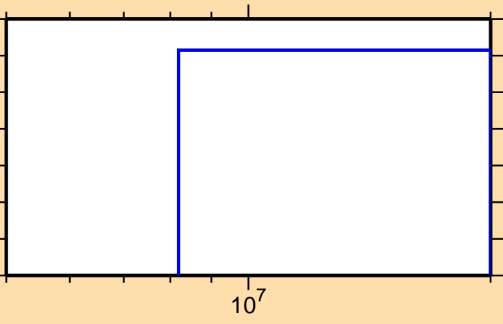
\sigma vs. E for ^{159}\text{Ho}(n,2np)
