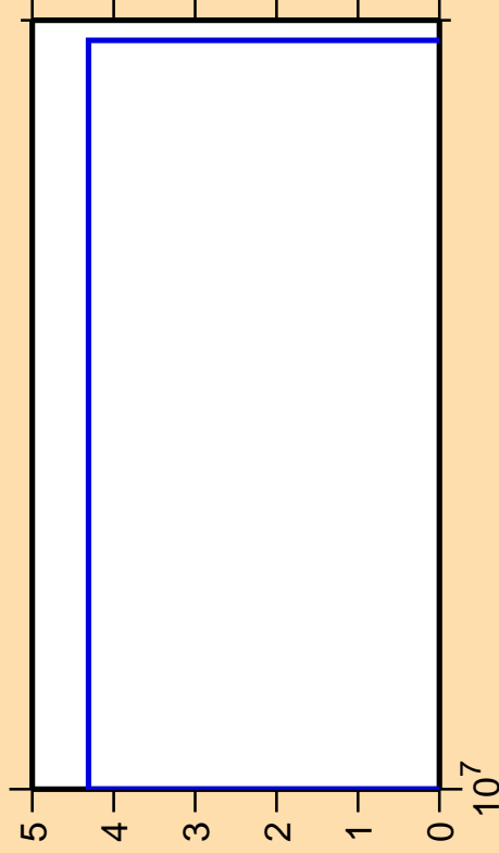
\Delta\sigma/\sigma vs. E for ^{160}\text{Ho} (mt 45)
