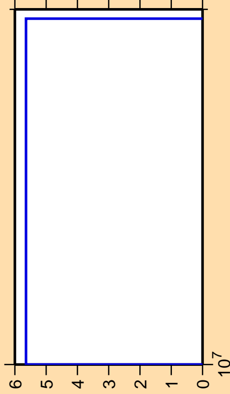
\Delta\sigma/\sigma vs. E for ^{160}\text{Ho}(\text{mt117})
