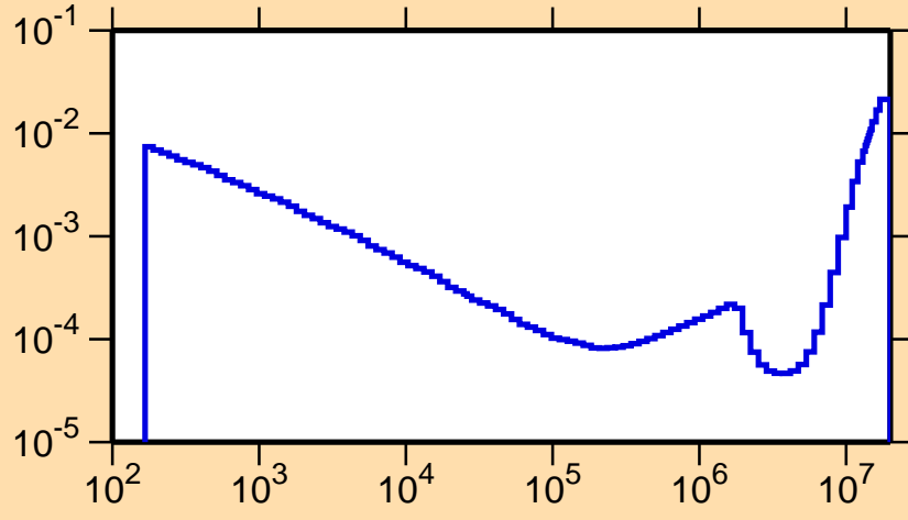
\sigma vs. E for ^{160}\text{Ho}(n,\alpha)
