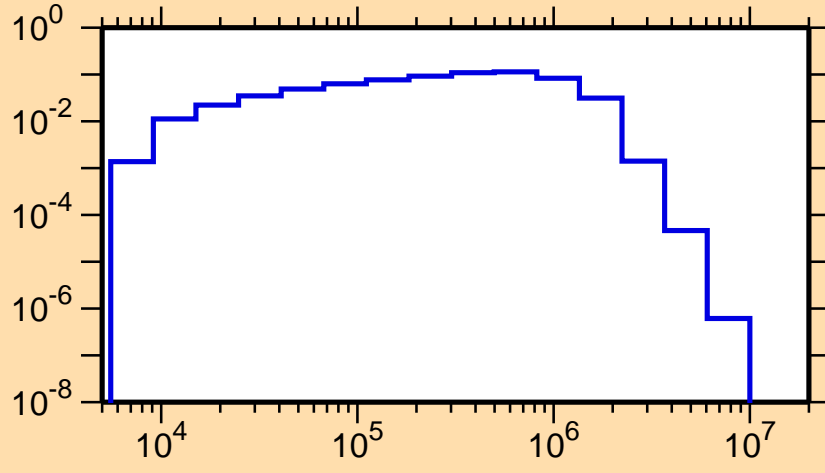
\sigma vs. E for ^{160}\text{Ho}(n,n_2)
