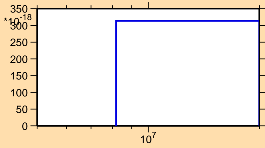
\sigma vs. E for ^{160}\text{Ho}(n,\text{pt})
