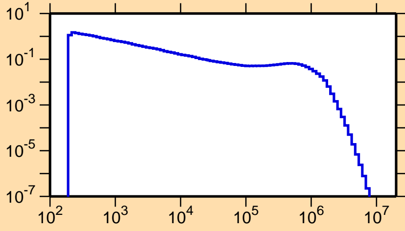
\sigma vs. E for ^{160}\text{Ho}(n,n_4)
