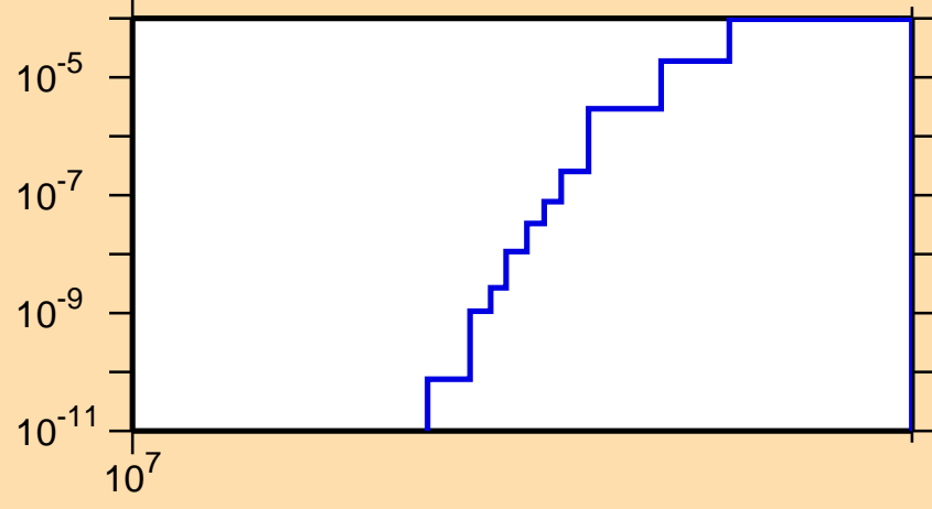
\sigma vs. E for ^{160}\text{Ho}(n,2np)
