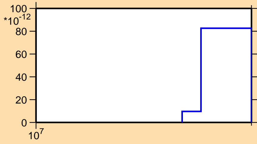
\sigma vs. E for ^{160}\text{Ho} (mt 45)
