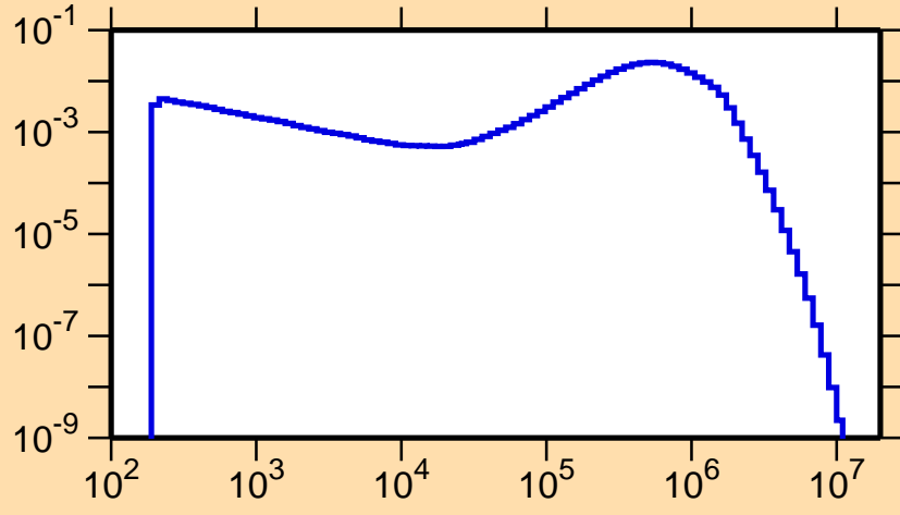
\sigma vs. E for ^{160}\text{Ho}(n,n_1)
