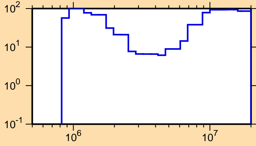
\Delta\sigma/\sigma vs. E for ^{160}\text{Ho}(n,n\text{cont.})
