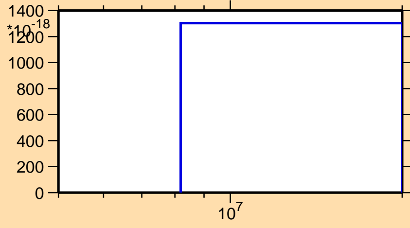
\sigma vs. E for ^{160}\text{Ho}(n,pd)
