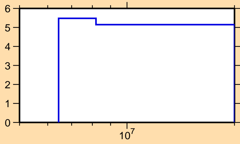
\Delta\sigma/\sigma vs. E for ^{160}\text{Ho}(n,\text{tot.})
