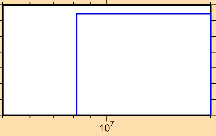
\sigma vs. E for ^{160}\text{Ho}(n,\text{He3})
