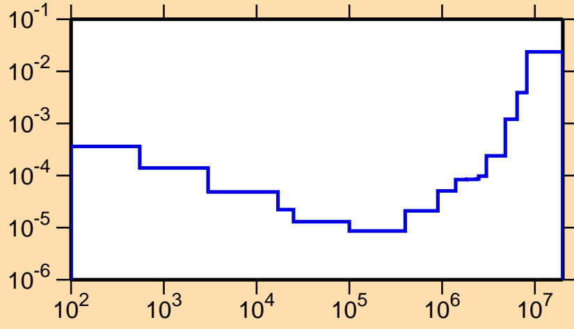
\sigma vs. E for ^{160}\text{Ho}(n,p)
